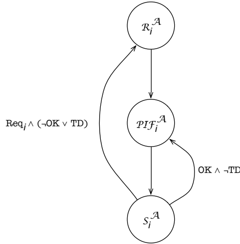
Figure 6.1: \text{TRANS1}_{\mathcal{A}}
