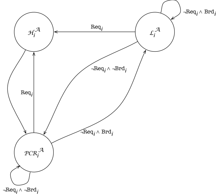
Figure 6.2: \mathcal{SNAP}_i
