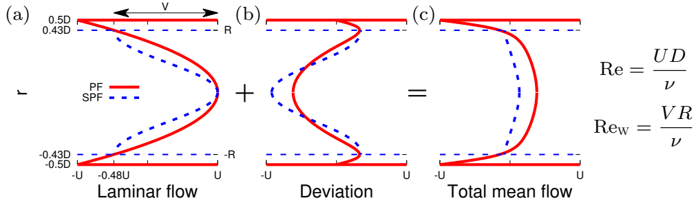
FIGURE 8. Stress-free pipe flow (SPF) seen as an approximation to the interior of pipe flow (PF). Shown are streamwise velocity profiles for PF (solid/red) and SPF (dashed/blue) in the uniformly turbulent regime (PF: Re = 3000 and SPF: Re_w = 1900 ). Plotted are (a) laminar flow, (b) deviation of mean turbulent profile from laminar flow, and (c) mean turbulent profile. The r -scale of SPF is non-dimensionalised using R = 0.86D/2 to align its stress-free boundaries (dashed horizontals) with extrema of PF deviation profile in (b). SPF velocities are likewise scaled by V = 2 \cdot 0.86^2 U so that both flows in (a) have the same average laminar shear. Data are from simulations of 2000 advective time units for pipes of length 5D .
