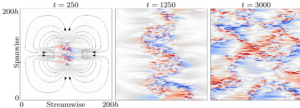
FIGURE 5. Growth of a turbulent spot in model Waleffe flow at \text{Re} = 160 . The flow is initialised with a poloidal vortex and subsequent evolution is visualised by streamwise velocity at the midplane. At early times ( t = 250 ), a large-scale quadrupolar flow dominates as shown by streamlines of the y -averaged flow (contour lines, only plotted away from the spot for visibility). By t = 1250 bands begin to develop and form a zigzag across the domain. The bands continue to grow, and by t = 3000 a complex array of bands fills the domain.
