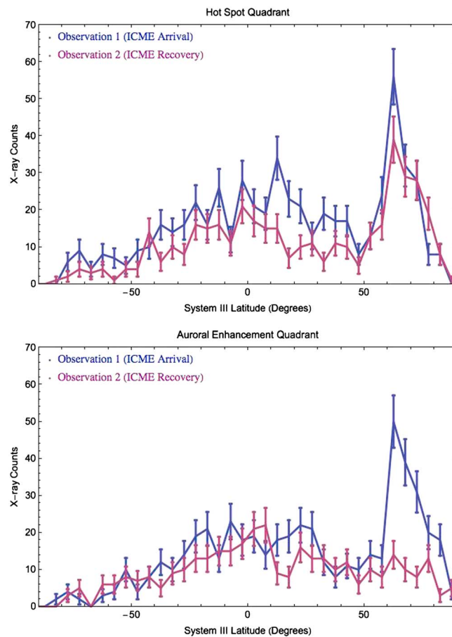
Figure 4. Number of events in 5° latitude bins during the first (blue) and second (red) observations. (top) Hot Spot Quadrant with S3 longitudes 90° – 180°. (bottom) Auroral Enhancement Quadrant with longitudes 180° – 270°. For the Auroral Enhancement Quadrant, emission above 60° latitude is up to 5 times brighter in the first observation than the second. Error bars are calculated from Poisson statistics. At the time of maximum visibility, each quadrant above 60° latitude had a projected area of ~3% of the total observable Jovian disk.
