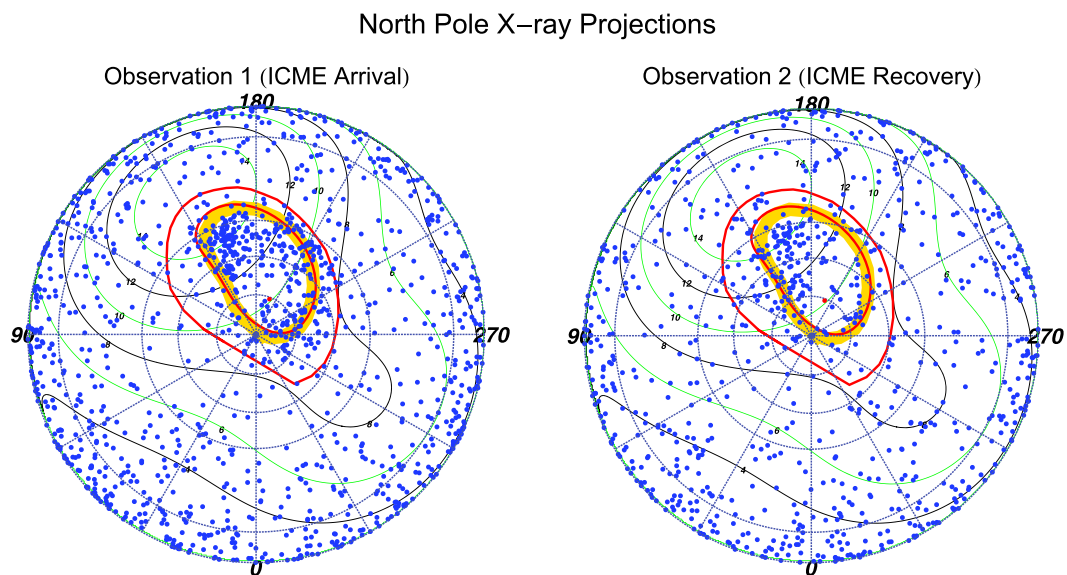
Figure 3. System III (S3) coordinate projections onto Jupiter’s geographic north pole (plot center) for the (left) first observation, during which the ICME arrived at Jupiter, and the (right) second observation, 1.2 days later. Lines of constant Jovian S3 longitude radiate outward from the pole, increasing clockwise in increments of 30° from 0° at the bottom of the projection. Concentric dotted circles outward from the pole represent lines of 80°, 70°, 60°, and 30° latitude. The alternate green and black contours indicate VIP4 model magnetic field strength in Gauss. The outer red oval is the Grodent et al. [2008] contour of Io’s footprint (5.8 R_J ). The inner red contour is the footprint for the 30 R_J field line from Vogt et al. [2011] mapping using the Grodent et al. [2008] anomaly model. The thick orange contour is the average location of the UV main oval from two HST observation campaigns in 2007 [ Nichols et al. , 2009]. The projections show more X-ray events in the hot spot (160°–180° S3 longitude, 60°–70° latitude) during the first observation than the second. The events appear to spread from the hot spot into the region from 150° to 160°. More clearly identifiable is the bright change in emission in the Auroral Enhancement Quadrant (180°–270° S3 longitude, 55°–90° latitude). The distribution of this emission is not only enhanced in the main oval but also poleward of this and at lower latitudes near Io’s magnetic footprint.
