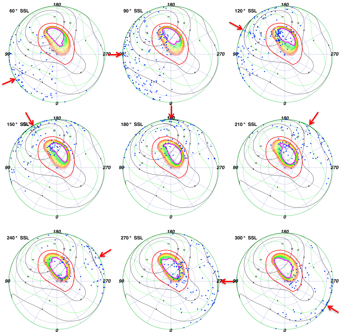
Figure 10. S3 polar projections of the first observation, binned based on subsolar longitude (SSL). Vogt et al. [2011] expanded magnetosphere models are plotted onto the polar projections. Throughout the observation, emission appears to exhibit a local time dependence and may follow the open-closed field line boundary. The time bins at 270° and 300° SSL show the auroral enhancement event. Each dot is an X-ray photon. For further plot details see Figure 9.
