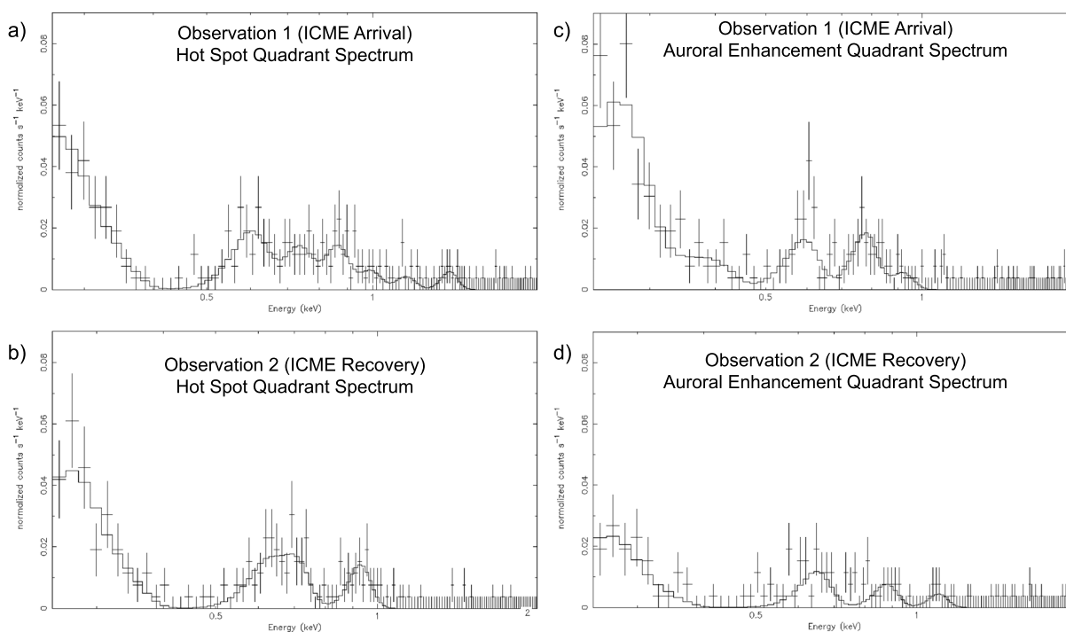
Figure 6. The northern auroral zone spectra for the (a, c) first and (b, d) second observations. The Hot Spot Quadrant spectra are in Figures 6a and 6b, while the Auroral Enhancement Quadrant spectra are in Figures 6c and 6d. The data have been fitted with a combination of lines with half widths fixed at 20 eV.
