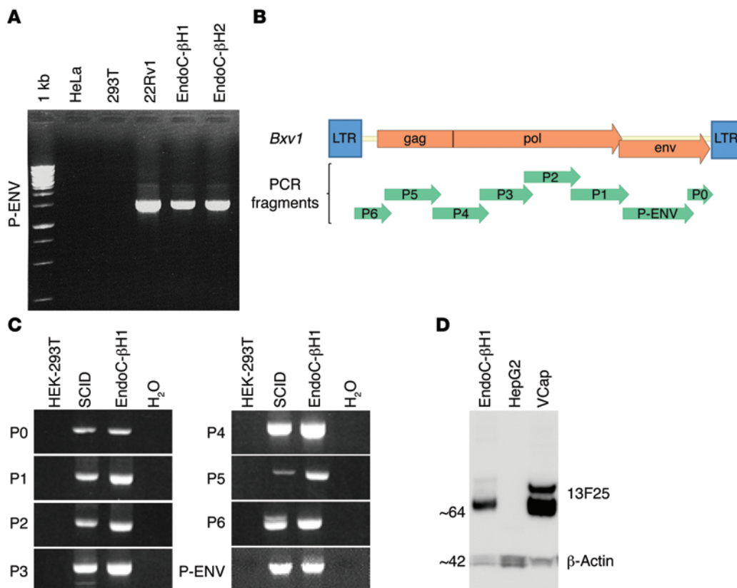
Figure 2. Bxv1 genome is integrated in EndoC-βH1/2 cells and SCID mice. (A) The sequence encoding the envelope protein from a broad range of xenotropic MuLV was amplified from genomic DNA from the indicated cell lines to generate the envelope protein-encoding fragment (P-ENV) PCR product (see B). HeLa and 293T cells are negative controls. (B) Position of the 8 PCR products covering the Bxv1 sequence. P0, primer set 0. (C) Amplification of Bxv1 genome using the 8 overlapping PCR fragments showing amplification in EndoC-βH1 cells and in SCID mice. Results are representative of 3 independent experiments. (D) Western blot showing that VCaP and EndoC-βH1 lysates are positive for 13F25 ( n = 6 ). See complete unedited blots in the supplemental material.
