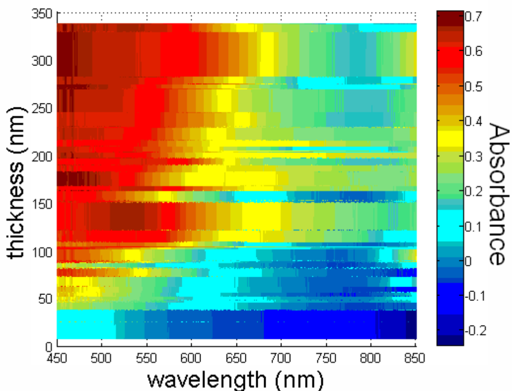
Figure 4. Experimental absorbance of individual supracrystals of different heights, for wavelength between 450 nm and 850 nm.
