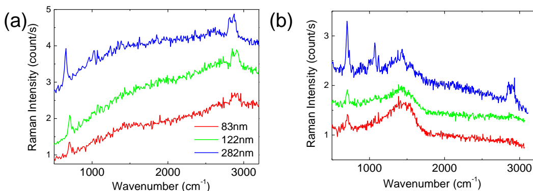
Figure 6. SERS spectra of the dodecanethiolate molecules coating the silver nanocrystals performed on three individual supracrystals having different heights h_{\text{supra}} (red: 83 nm, blue: 282 nm, green: 122 nm) for two laser excitation wavelengths. (a) 514 nm, laser power 20 \mu\text{W} and (b)
