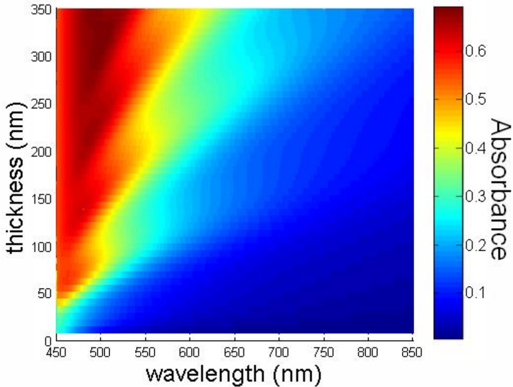
Figure 5. Simulated absorbance for different supracrystals heights h_{\text{supra}} , for wavelength between 450 nm and 850 nm with the following parameters: q = 0.312 , \epsilon_m = 2.16 , \Gamma = 1.5 . See text for details.
