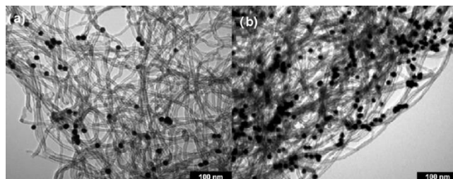
Figure 6. TEM images of MWCNT samples covered with gold metallic nanoclusters (10 nm) deposited by the atmospheric plasma treatment using (a) Ar and (b) Ar/O 2 mixture. Flow rates were 30 \text{ L.min}^{-1} for Ar and 20 \text{ mL.min}^{-1} for O 2 .
