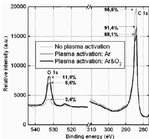
Figure 1. XPS spectra core levels of O 1s and C 1s of MWCNTs: not activated, plasma-activated with an argon flow rate of 30 L.min -1 and plasma-activated with an argon flow rate of 30 L.min -1 and oxygen flow rate of 20 mL.min -1 . The RF plasma power was 80 W.
