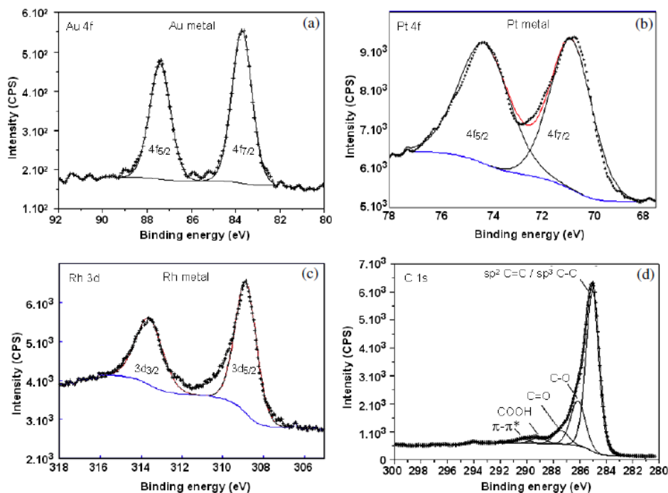
Figure 4. Fitted core levels for (a) Au 4f, (b) Pt 4f, (c) Rh 3d and (d) C 1s peaks after the atmospheric argon plasma treatment. Note that the presented fitted C 1s level corresponds to Au/MWCNT sample characterization. The fitted C 1s level is similar for the Pt/MWCNT and Rh/MWCNT samples.
