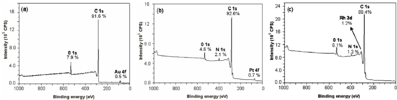
Figure 3. Survey XPS spectra recorded on (a) Au/MWCNTs, (b) Pt/MWCNTs and (c) Rh/MWCNTs after atmospheric Ar plasma treatment.
