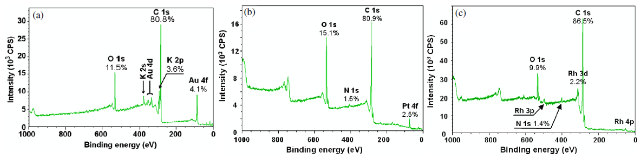
Figure 5. Survey XPS spectra recorded on (a) Au/MWCNTs, (b) Pt/MWCNTs and (c) Rh/MWCNTs after the argon-oxygen plasma treatment. The flow rates were 30 L. \text{min}^{-1} for argon and 20 mL. \text{min}^{-1} for oxygen.
