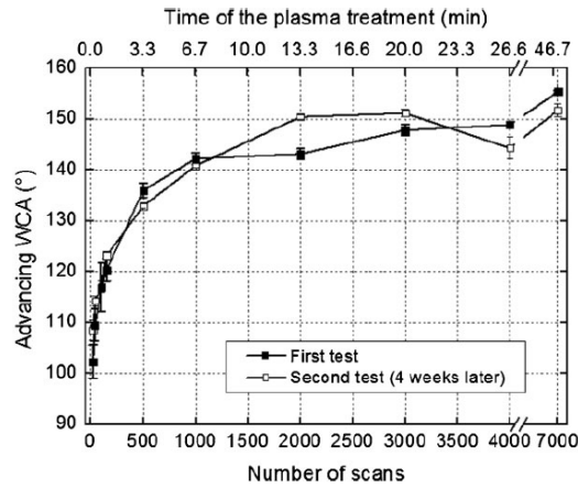
Figure 13. WCA ageing study of PTFE samples treated by a He–O 2 post-discharge ( F(\text{He})=15 \text{ L/min} , F(\text{O}_2)=100 \text{ mL/min} , P_{\text{RF}}=90 \text{ W} , v_s=25 \text{ mm/s} , g_s=1 \text{ mm} , L_s=20 \text{ mm} ).
