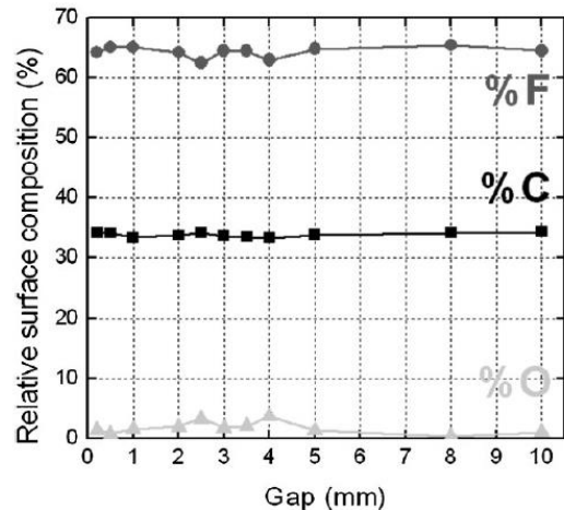
Figure 5. Surface elementary compositions of He-O 2 plasma-treated PTFE samples ( L_s=10\text{mm} , v_s=25\text{ mm/s} , N_s=1000 , F(\text{He})=15\text{ L/min} , F(\text{O}_2)=100\text{ mL/min} , P_{RF}=90\text{ W} ).
