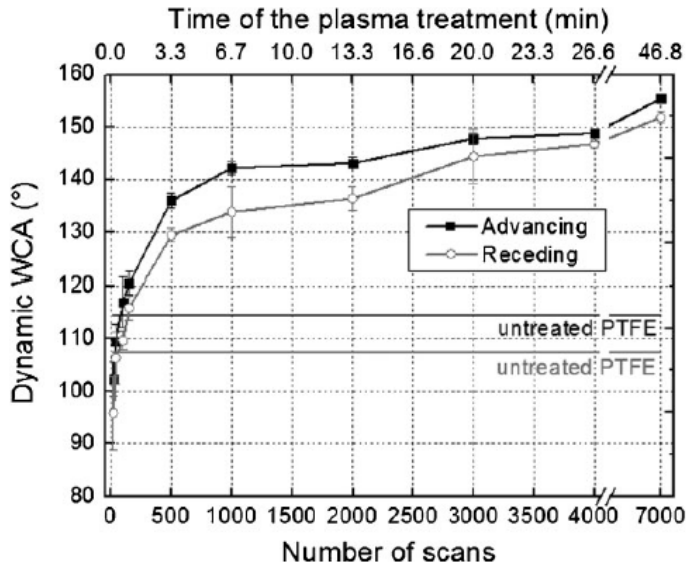
Figure 2. WCA measured on plasma-treated PTFE samples, versus the number of scans ( L_s=10\text{mm} , v_s=25\text{ mm/s} , g_s=500\text{ mm} , F(\text{He})=15\text{ L/min} , F(\text{O}_2)=100\text{ mL/min} , P_{RF}=90\text{ W} ). The top X-axis gives the corresponding exposure time for the plasma treated samples.
