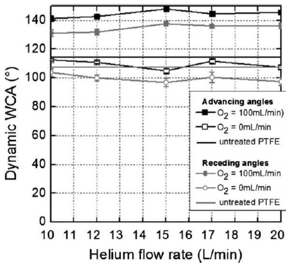
Figure 7. Influence of the helium flow rate on the WCA ( v_s=25\text{ mm/s} , g_s=1\text{ mm} , L_s=10\text{ mm} , N_s=1000 , P_{RF}=90\text{ W} and F(O_2)=0\text{--}100\text{ mL/min} ).
