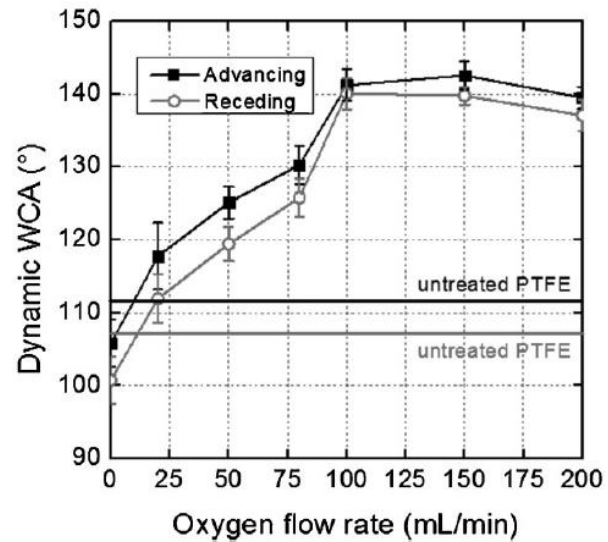
Figure 8. Influence of the oxygen flow rate on the plasma-treated PTFE WCA for L_s=10\text{ mm} , g_s=500\text{ mm} , N_s=800 , v_s=25\text{ mm/s} , F(\text{He})=15\text{ L/min} , P_{RF}=90\text{ W} .
