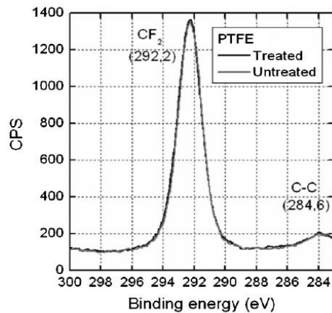
Figure 6. High resolution C 1s spectrum of He-O 2 plasma-treated PTFE for g_s=500\text{mm} , L_s=10\text{ mm} , v_s=25\text{ mm/s} , N_s=1000 , F(\text{He})=15\text{ L/min} , F(\text{O}_2)=100\text{ mL/min} , P_{\text{RF}}=90\text{ W} .
