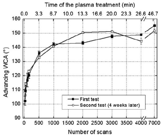
Figure 13. WCA ageing study of PTFE samples treated by a He–O 2 post-discharge ( F(\text{He})=15 \text{ L/min} , F(\text{O}_2)=100\text{mL/min} , P_{\text{RF}}=90\text{W} , v_s=25\text{mm/s} , g_s=1\text{mm} , L_s=20\text{mm} ).
