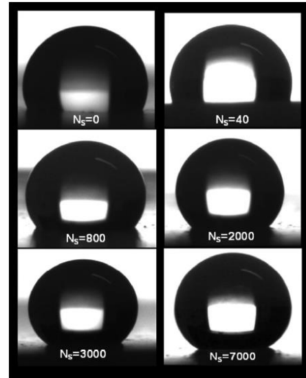
Figure 3. Droplets of ultra-pure water deposited on different plasma-treated PTFE surfaces; each surface being exposed to a specific number of scans. ( L_s=10\text{mm} , v_s=25\text{ mm/s} , g_s=500\text{ mm} , F(\text{He})=15\text{ L/min} , F(\text{O}_2)=100\text{ mL/min} , P_{RF}=90\text{ W} ).
