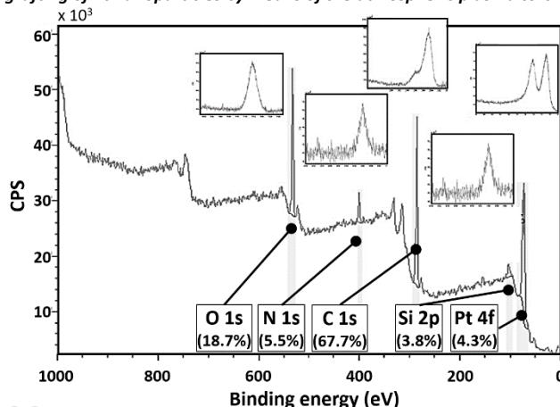
Figure 6. XPS survey of Pt grafted on glassy carbon after ultrasonication with insets showing narrow scans of the elements.
