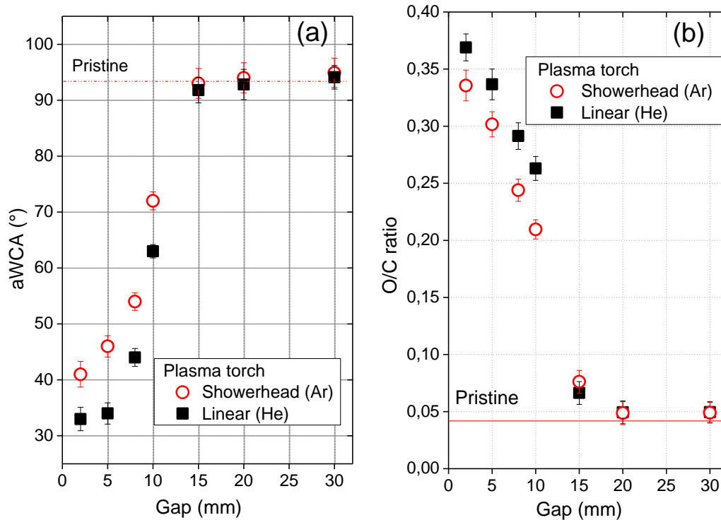
Figure 4. Variation of (a) aWCA and (b) O/C ratio of LDPE surfaces treated by the linear and showerhead plasma torches vs. the gap for P_{RF}=90W , t = 30 s, \Phi(O_2) = 0 mL/min.
