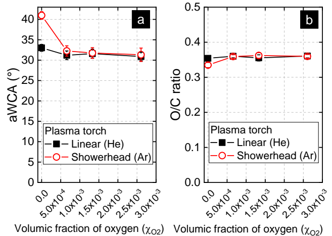
Figure 6. Variations of the (a) aWCA and (b) O/C ratio vs. volume fraction of oxygen ( P_{RF} = 90\text{W} , t = 30\text{s} , g = 2\text{mm} ) for LDPE surfaces treated by the linear and showerhead plasma torches.
