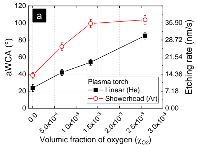
Figure 6. Variations of the (a) aWCA and (b) O/C ratio vs. volume fraction of oxygen ( P_{RF} = 90\text{W} , t = 30\text{s} , g = 2\text{mm} ) for LDPE surfaces treated by the linear and showerhead plasma torches.
