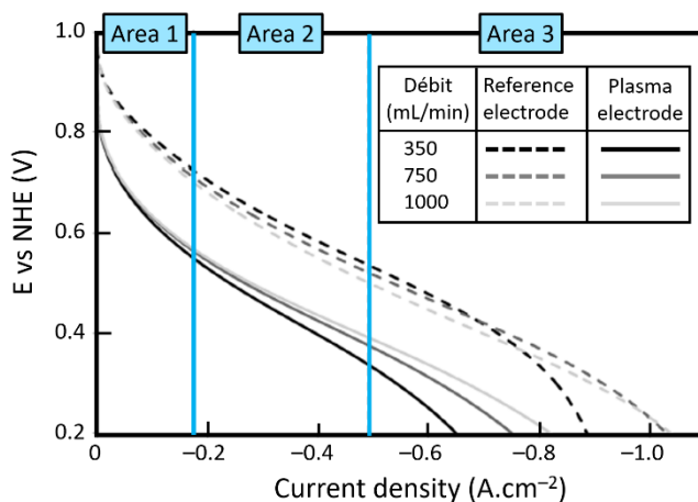
Figure 10. Dynamical polarization curves of the mono-fuel cell containing the reference electrode and the plasma electrode as cathode realized in the following conditions ( A=25 \text{ cm}^2 , open configuration, gap = 3 mm, \text{Ar} = 30 \text{ L}\cdot\text{min}^{-1} , 60W, 300 s).
