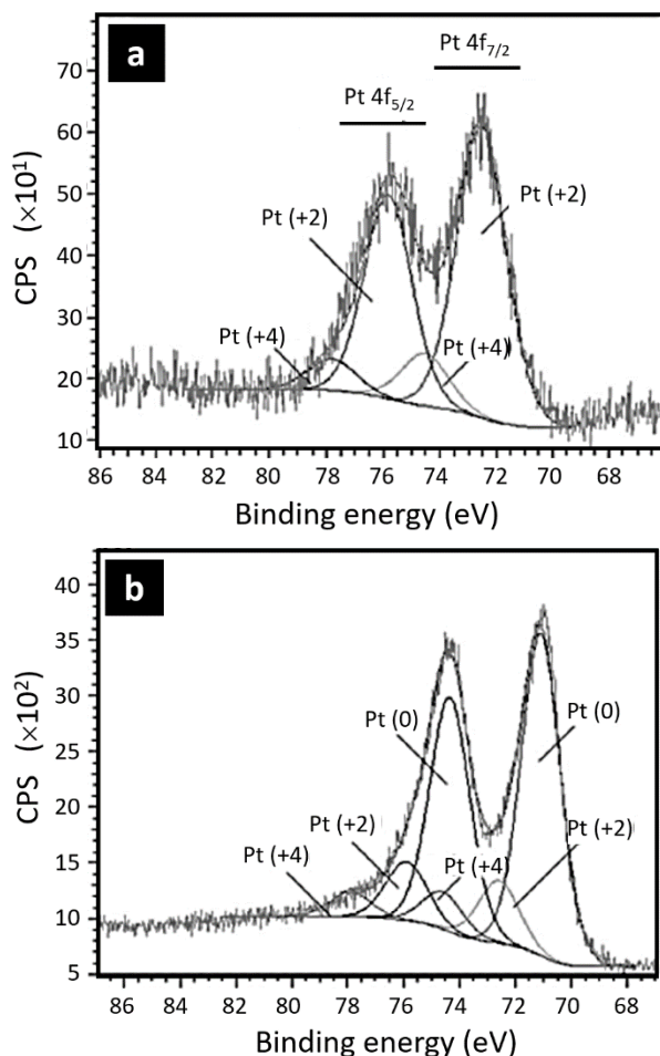
Figure 4. Comparison between Pt 4f spectra for a plasma treatment of the CB/[Pt(acac) 3 ] mixture during 300 s (60 W, 30 L.min -1 Ar, gap = 10 mm) (a) in the "open configuration" and (b) in the "confined configuration".
