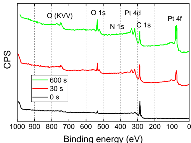
Figure 2. Survey scan spectra of the CB/[Pt(acac) 2 ] untreated mixture, the mixture treated during 30 and 600 s ( P = 60 W, Ar flow rate = 30 \text{ L} \cdot \text{min}^{-1} , gap = 3 \text{ mm} ).
