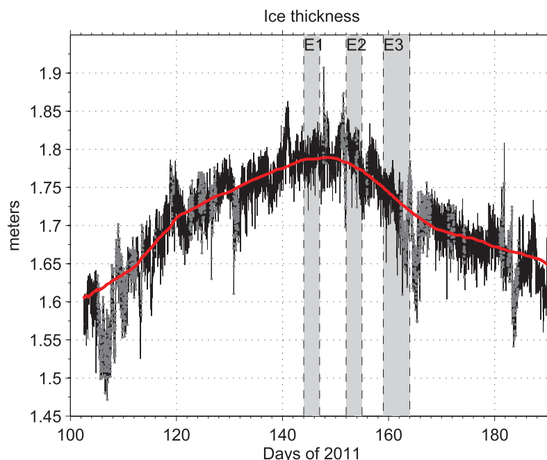
Figure 8. Evolution of ice thickness as estimated by the Ice-T. Black line denotes the raw estimate, while the red line shows low-pass filtered ice thickness with a cutoff period of 20 days. Gray dots mark estimates with larger uncertainty (see full description in section 3.4).
