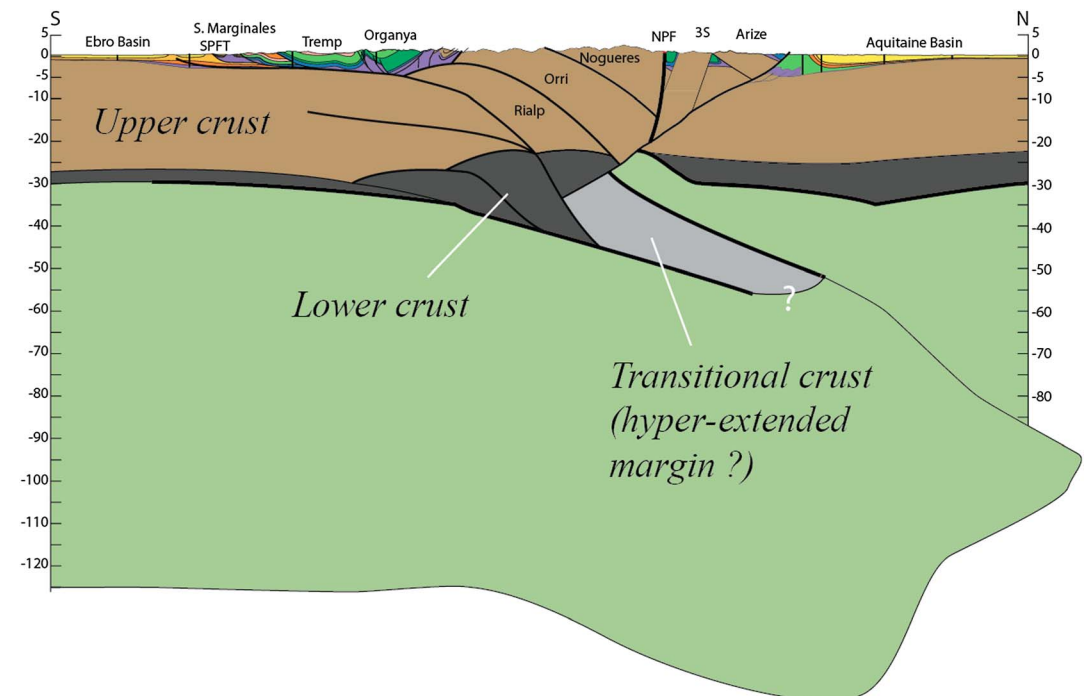
Figure 2. Lithosphere-scale section across the Pyrenees (see location in Figure 1). This interpretation accounts for a recent cross section proposed by Mouthereau et al. [2014] that was updated considering the migration of teleseismic P wave data from Chevrot et al. [2015]. This version is aimed at accounting for the subduction of the distal, hyperextended margin at depth. Note that the thickening of the lower crust reflects the thickening of the Iberia proximal margin and forms the main part of the mountain root.
