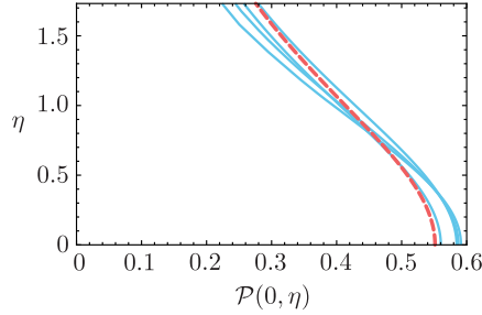
FIGURE 16. Pressure along the axis \bar{r} = 0 obtained with Gerris for \bar{t} = 5 \times 10^{-3} , 10^{-2} , 5 \times 10^{-2} and 10^{-1} (same as in Fig. 10 right) represented in the self-similar space ( \text{Re} = 5000 and \text{We} = 250 ). The red dashed line is the analytical solution for \mathcal{P}(\xi = 0, \eta) . Fluctuations of the pressure around the theoretical prediction is to be related with numerical projections errors.
