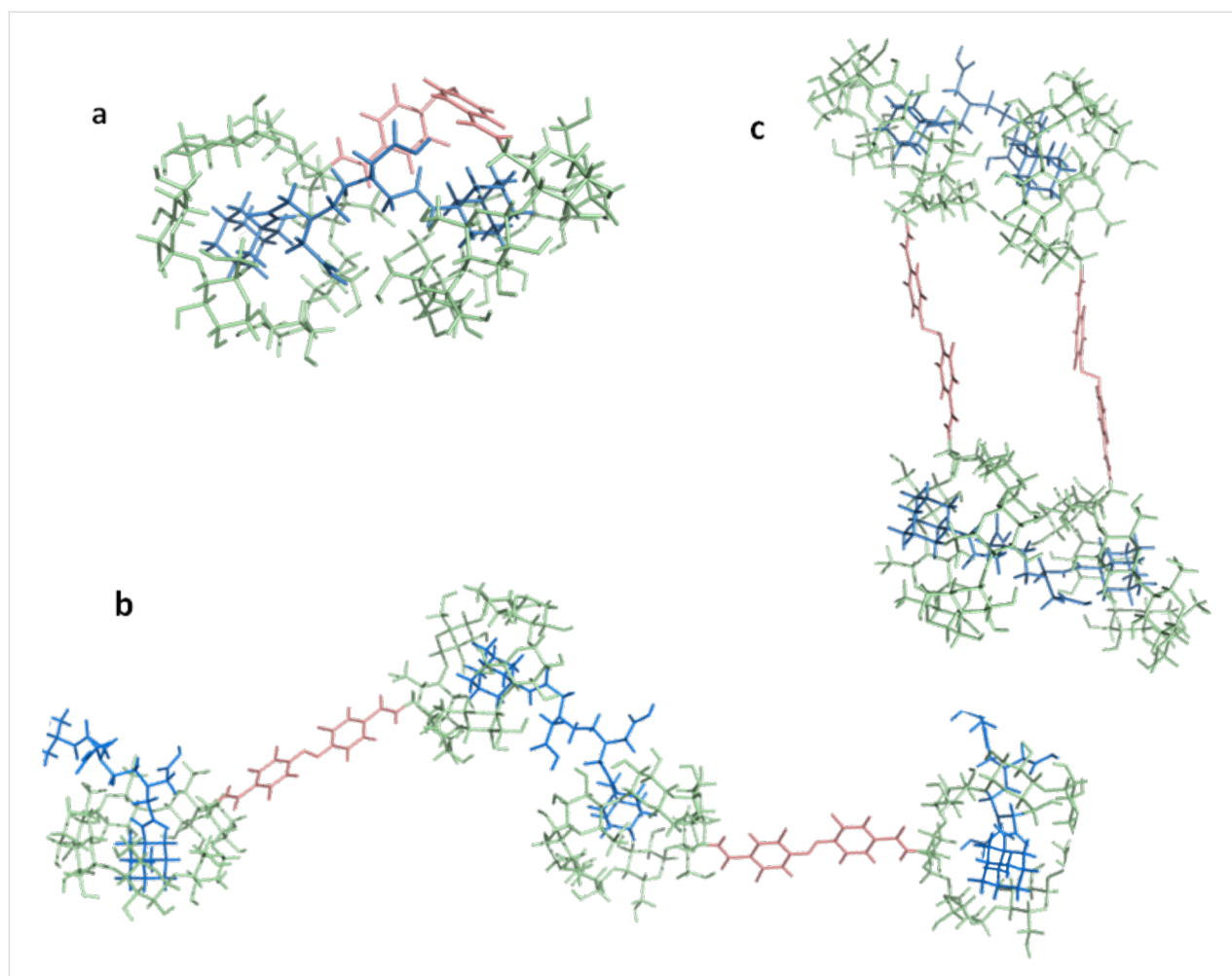
Figure 8: Proposed structures of inclusion complexes with the ditopic host AZO-CDim 1 and the ditopic guest ADAAdim 4 after minimization by molecular modeling methods: (a) 1:1 chelate-type complex with AZO-CDim 1 in its cis configuration; linear (b) and cyclic (c) supramolecular polymers with AZO-CDim 1 in its trans configuration.
