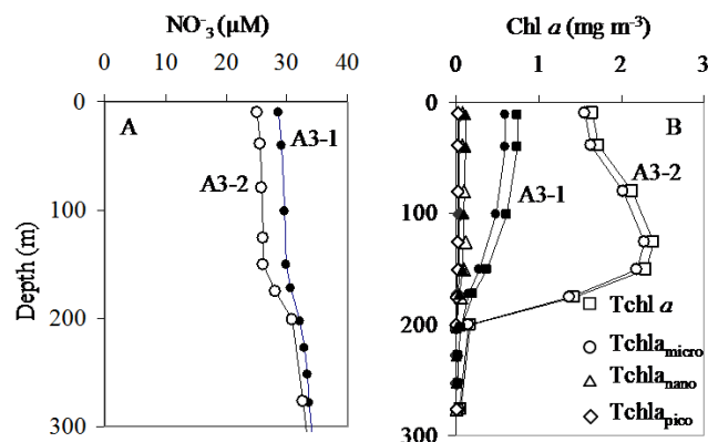
Figure 3. Vertical distribution of the concentration of \text{NO}_3 (A); total Chl a ( T_{chl a} ), and T_{chl a} associated with micro- ( T_{chl a \text{ micro}} ), nano- ( T_{chl a \text{ nano}} ), and picophytoplankton ( T_{chl a \text{ pico}} ) (B). The filled symbols indicate pre-bloom stage; the hollow symbols indicate early bloom stage.
