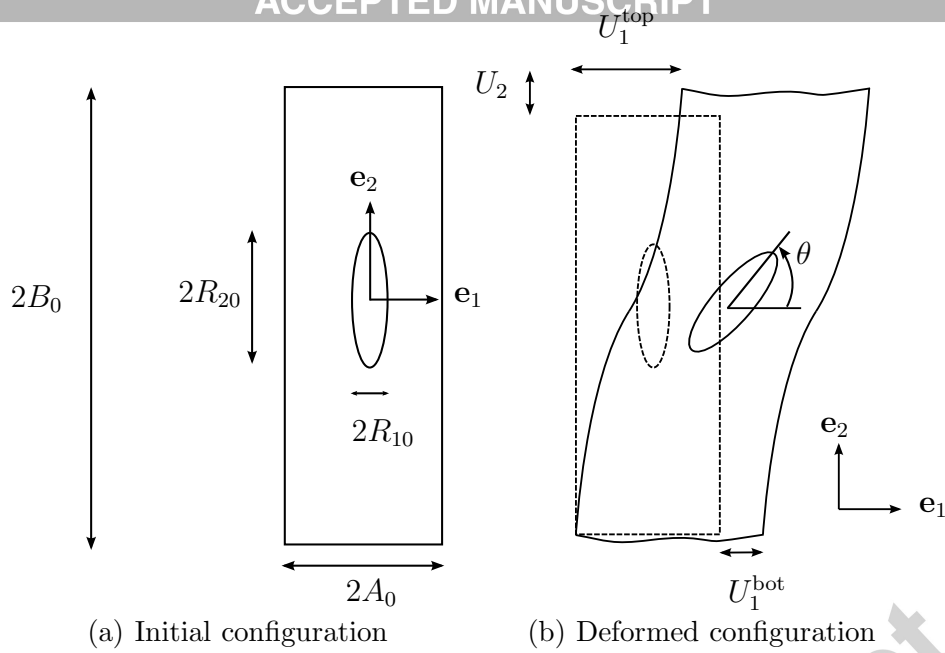
Fig. 5. Elementary cell containing an initially elliptical cylindrical void (after Tvergaard (2015a))
