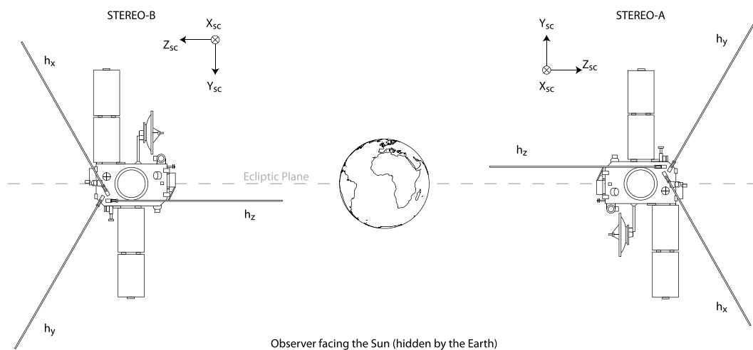
Figure 1. STEREO antenna orientation as seen from an observer facing the Sun (hidden by the Earth in the scheme). h_{x,y,z} display the physical antenna, while (X,Y,Z)_{sc} shows the orientation of the spacecraft reference frame.
