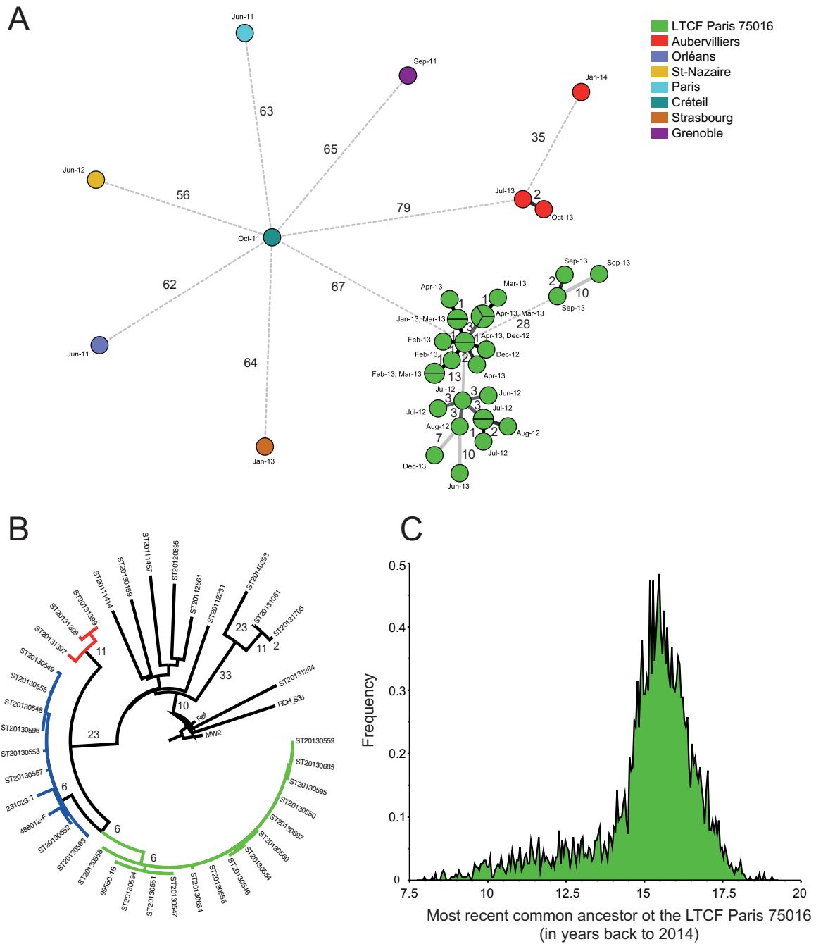
FIG 5 Evolutionary relationships of the strains from an outbreak at a long-term care facility (LTCF) in the Paris area. (A) Minimum spanning tree based on SNP data. Circle sizes are a function of the number of strains with the same genotype. Dashed lines correspond to links with >25 SNPs; thin lines correspond to links with <25 SNPs, and thick lines correspond to links with ≤10 SNPs. Dates of isolation are indicated. Colors represent the geographical or epidemiological origins according to the key. (B) ML tree based on the alignment of 488 SNPs of the dominant French lineage. Numbers of SNPs are mapped on the branches. Strains from the outbreak group in three clusters colored green, blue, and red. (C) Posterior distribution of the Paris LTFC TMRC generated with the BEAST algorithm. The common ancestor (median) appeared in Europe in 1998 (95% highest posterior density, 1996 to 2003).
