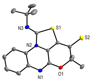
Figure 7. ORTEP representation of imino-thiazole 18 at 50 % probability. Hydrogen atoms are omitted for clarity.
