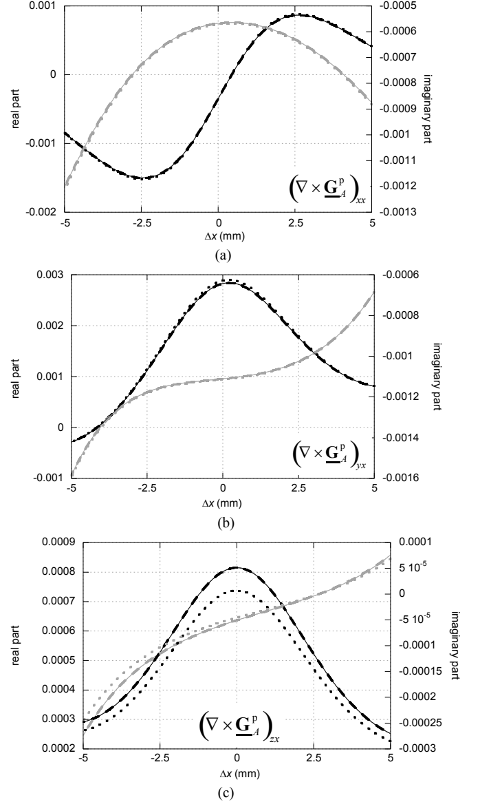
Fig. 4. Green's functions comparisons (the relevant potential is indicated in the figure): real parts (black lines) and imaginary parts (gray lines). The structure is that of Fig. 2. The potentials are computed along the segment -p/2 < \Delta x < p/2 , \Delta y = p/2 , and z' = 0 . The Bloch wavenumber is k_{x0} = -0.5k_0 - j0.2k_0 (the n = 0 harmonic is radiating and is proper [6], [11]). Potentials computed with (continuous lines) and without (dashed lines) acceleration at z = 0.1 mm (off plane) and with acceleration (dotted lines) at z = 0 (on plane). (Note: the terms plotted are unitless.)
