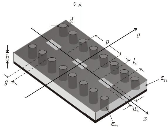
Fig. 1. Example of a structure requiring the computation of the vertical periodic potentials and the curls of dyadic periodic potentials: A substrate integrated waveguide structure synthesized by two rows of cylindrical dielectric inclusions in a host dielectric layer embedded between two metallic plates. Periodic slots are etched on the top metal plate.
