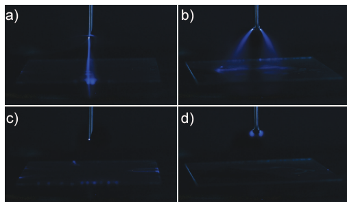
Figure 1: Photographs of the DC corona discharges in air with a hypodermic injection needle as HV electrode (clipped for water electro spray b, d) and a glass cover slide on a copper grounded electrode: a) positive corona, b) positive corona with water electro spray, c) negative corona, d) negative corona with water electro spray (4 s exposure time).
