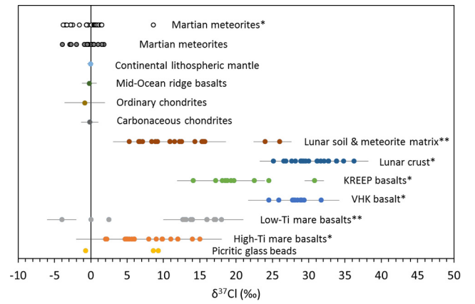
Fig. 7. Plot comparing the chlorine isotopic compositions of different objects in the Solar System. All of the data available for lunar samples (Sharp et al., 2010; Treiman et al., 2014; Tartèse et al., 2014b; Boyce et al., 2015; this study) have been plotted together with their individual uncertainties. * data from the in situ analyses of apatite and ** data included from both in situ analyses of apatite and bulk Cl isotope measurements. Also plotted are the new data Cl isotope measurements of martian meteorites from Williams et al. (in press), both bulk measurements (grey symbols) and in situ apatite measurements (denoted by *). The average \delta^{37}\text{Cl} values for the Earth's continental mantle, mid-ocean ridge basalts, Earth, ordinary and carbonaceous chondrites have been plotted with the uncertainties representing the 2\sigma standard deviation of the literature values (Sharp et al., 2013a).
