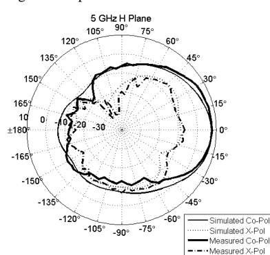
Fig. 11. Realized gain in H-plane at 5 GHz.
