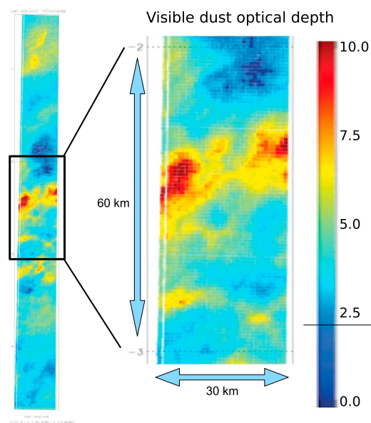
Figure 1. Column dust optical depth at 1\text{ }\mu\text{m} observed by OMEGA in Terra Meridiani. The zoomed area is located at coordinates ( 25^\circ\text{E}, 2.5^\circ\text{S} ). Values below the horizontal line in the color bar cannot be considered as reliable. Adapted from Määttänen et al. [2009] with permission.
