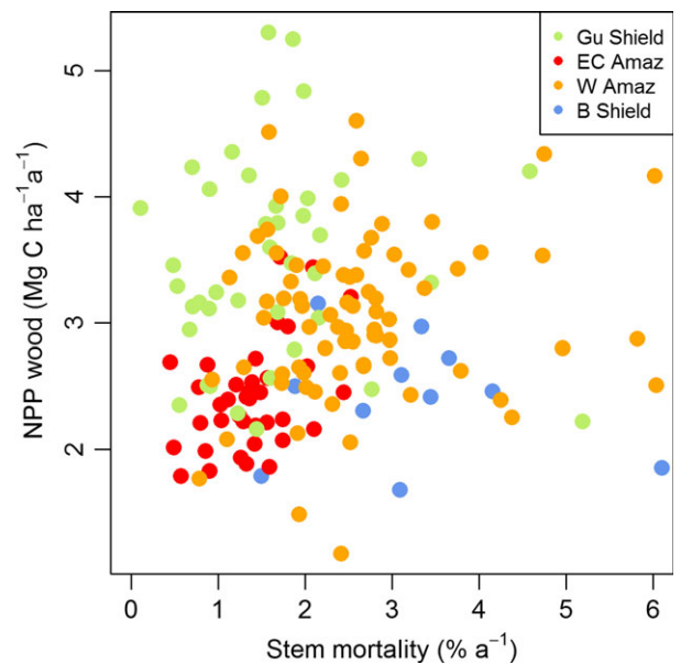
Fig. 3 Relationship between woody net primary productivity (NPP) and stem mortality rates for 167 forest plots in four regions of Amazonia.
