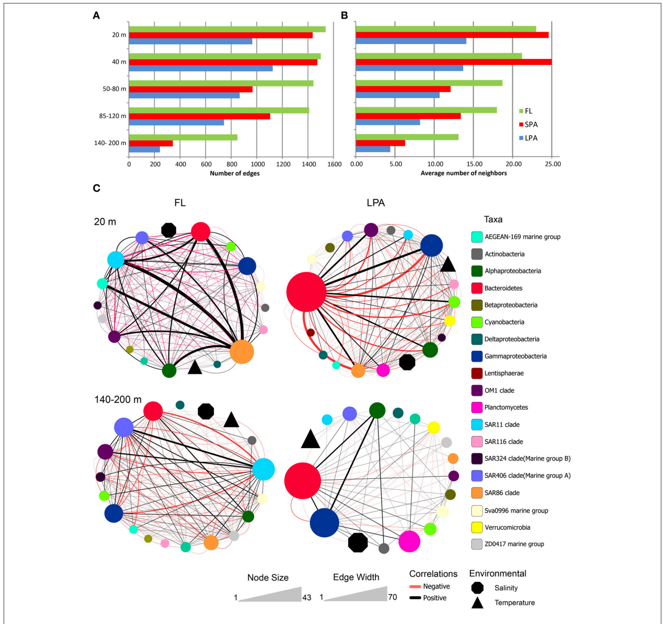
FIGURE 6 | Bacterioplankton co-occurrence networks. Network analysis was performed at the OTU level for each depth layer and size fraction of the plankton. Selected topological parameters of the networks are plotted: (A) Number of edges in each network and (B) average number of neighbors per node. See Tables S8–S10 for the full set of network parameters. (C) The four most extreme networks are displayed: The 20 and 140–200 m depth layer (top to down) of the FL and LPA communities (left to right), respectively. In order to better display co-occurrence patterns OTUs were grouped at different taxonomic level (known marine clades as well as classes and phyla). The size of each oval (node) indicates the number of OTUs belonging to that taxonomic group, while the size of environmental parameters (temperature and salinity) was arbitrary defined. Lines connecting two nodes represent a group of strong ( R > 0.6 ) and significant correlations ( p < 0.05 ). Black lines indicate a positive correlation while red lines indicate a negative correlation. The width of each line exhibit the number of correlations occurring among the two connected nodes.
