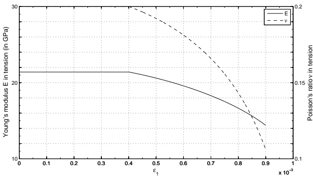
Figure 3. Uniaxial tension. Evolutions of Young's modulus and Poisson's ratio.
