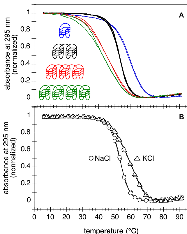
Figure 1. UV-melting profiles of (GGGTTA) 4m-1 GGG oligonucleotides. (A) Absorbance at 295 nm as a function of temperature of H21 ( m = 1 , blue line), H45 ( m = 2 , black bold line), H69 ( m = 3 , red line) and H93 ( m = 4 , green line) in 100 mM NaCl. (B) Absorbance at 295 nm as a function of temperature of H45 in 100 mM NaCl (circles) or KCl (triangles). Cooling and heating profiles are shown; they were normalized between the minimum and the maximum of absorbance. The conformation used to represent tandem G4s is speculative and for illustrative purpose.
