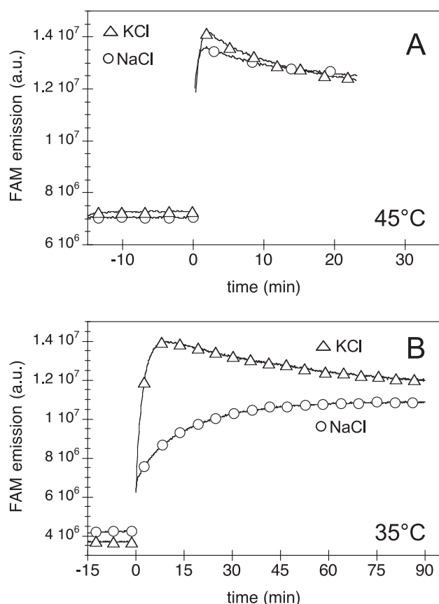
Figure 2. Opening kinetics of the molecular beacon in the presence of H45. Fluorescence emission of 0.2 \mu M molecular beacon MB alone ( t < 0 ) and in the presence of 0.8 \mu M H45 ( t > 0 ), in 100 mM NaCl (circles) or KCl (triangles), at 45°C (A) and at 35°C (B). Excitation wavelength: 470 nm; emission wavelength: 520 nm. The fluorescence intensity of the molecular beacon alone ( t < 0 ) depends on the temperature (about 7 \times 10^6 a.u. at 45°C and about 4 \times 10^6 a.u. at 35°C); this is because the FAM emission of the molecular beacon is proportional to the molecular beacon unfolded fraction, which increases with the temperature (Supplementary Figure S4).
