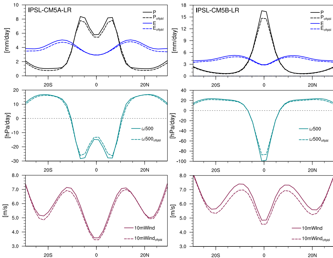
Figure 5. Aquaplanet annual mean changes ( offpbl aqua - aquaControl difference averaged over 3 years) in tropical precipitation and circulation predicted by the (left) IPSL-CM5A-LR and (right) IPSL-CM5B-LR models: solid lines correspond to the control aquaplanet simulation and dashed lines correspond to offpbl aqua simulations. (top) Zonal mean precipitation (black) and evaporation (blue). (middle) Zonal means of 500 hPa vertical velocity, \omega_{500} . (bottom) The zonal means of 10 m wind.
