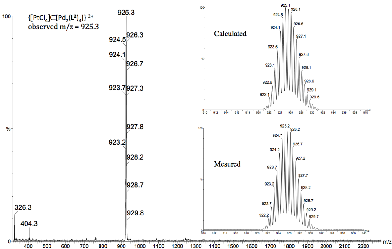
Figure 6. Calculated and observed isotope pattern for the intact metallocage [[PtCl_4] \subset Pd_2(L^2)_4][OTf]_2 ( 4 ).
