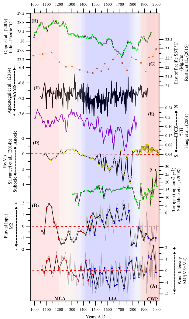
Figure 4. (a) Wind intensity ( M4/(M3+M4) ) anomaly reconstruction, (b) fluvial input ( M2 ) anomaly reconstruction on the continental shelf, and records of (c) terrigenous flux (total minerals) in Pisco continental shelf by Sifeddine et al. (2008), (d) OMZ activity (Re / Mo anomalies) negative values indicate more anoxic conditions (the axis was reversed) (Salvatteci et al., 2014b), (e) ITCZ migration (%Ti) (Peterson and Haug, 2006), (f) SAMS activity reconstruction ( \delta^{18}\text{O} Palestina Cave) (Apaéstegui et al., 2014), (g) eastern temperatures reconstruction (Rustic et al., 2015) and (h) Indo-Pacific temperatures reconstruction (Oppo et al., 2009).
