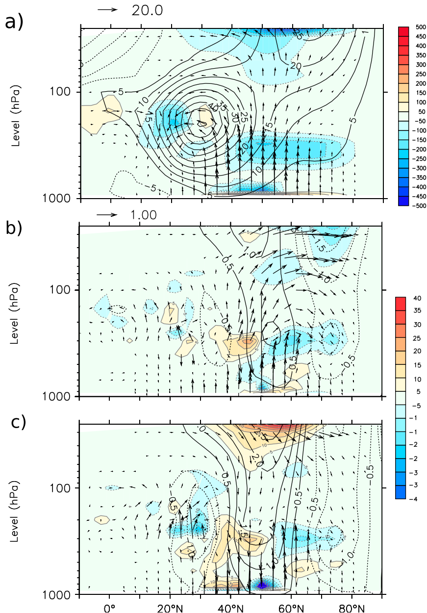
FIG. 11. The EP flux by planetary (zonal wavenumber k = 1-3 ) waves (arrows, \text{m}^2 \text{s}^{-2} ), its divergence (colors, \text{m} \text{s}^{-2} ), and zonal-mean zonal wind (contours, \text{m} \text{s}^{-1} ), for the 30-day period centered on 10 February, for (a) CTR climatology, (b) the \text{Atl}_{\text{ALL}} - \text{CTR} difference, and (c) the \text{Atl}_{\text{SST}} - \text{CTR} difference. Zonal averaging is over all longitudes. The scaling of Edmon et al. (1980) is used for the EP flux vectors.
