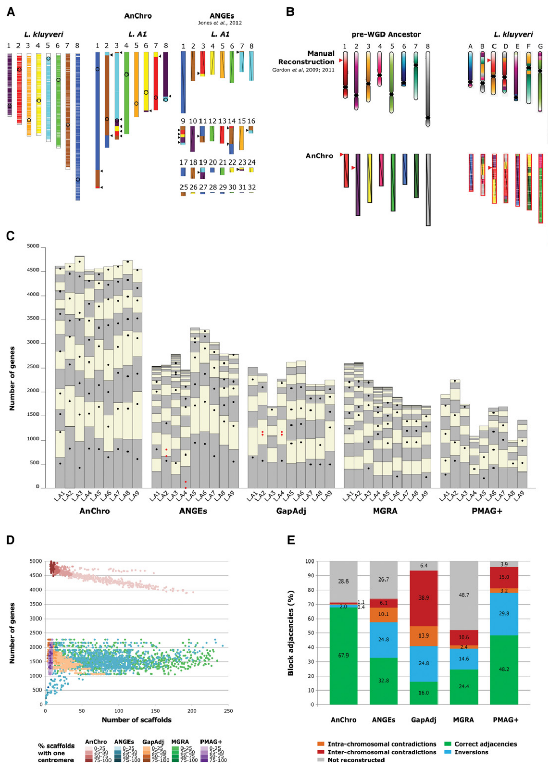
Figure 4. (A) Comparison between the two versions of the L. A1 ancestral genome reconstructed by AnChro and by ANGES (Jones et al. 2012). Chromosome painting representations of ancestral genomes are colored relatively to the L. kluyveri chromosomes. The black triangles indicate the same 12 ancestral adjacencies that resulted from six translocations identically reconstructed by the two tools. (B) Comparison between the manually reconstructed (Gordon et al. 2009, 2011) and the AnChro version of the pre-WGD ancestral genome relative to the L. kluyveri genome. The only inter-chromosomal difference between the two reconstructions is indicated by the red triangles. (C) Comparison of the nine Lachancea ancestors ( L. A1 to L. A9 ) reconstructed by AnChro , ANGES , GapAdj , MGRA , and PMAG+ . Syntenic blocks were computed with I-ADHoRe for the five reconstruction tools. For AnChro , a single default reconstruction is presented. Each column represents the ancestral chromosomes of a given ancestor as an alternation of gray and beige boxes, with size being proportional to the number of reconstructed ancestral genes. The small black circles indicate the centromere position. The small red circles indicate the centromere positions when an ancestral chromosome was reconstructed with two centromeres. (D) Ancestral genome reconstructions on simulated genomes. The figure presents 900 reconstructed ancestral genomes corresponding to nine different ancestors per simulation and 100 simulations, performed with AnChro (default reconstructions), ANGES , GapAdj , MGRA , and PMAG+ . Each genome reconstruction is represented by a dot. The quality of the reconstructions is assessed by three criteria: the number of ancestral scaffolds (ideally eight), the number of ancestral genes (ideally 5000), and the proportion of scaffolds per reconstruction with a single centromere (ideally 100%). (E) Average proportions of correctly and incorrectly reconstructed adjacencies for the 900 reconstructions obtained by the five tools. Incorrect adjacencies are decomposed in single block inversions and intra- and inter-chromosomal contradictions. The average proportion of adjacencies that were not reconstructed by the different software is also indicated.
