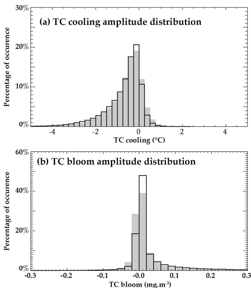
Figure 4. Normalized distributions of (a) SST and (b) chlorophyll responses under TCs (in 200 km radius, see text) in observations (shaded grey) and in the model (black). The x axis has been purposely limited to the main responses but outliers also exist in the distributions. The amplitude of the response refers to the signal averaged between days +2 to +5 from the cyclone passage for chlorophyll and from day +1 to +4 for the SST, relative to the average situation between 10 and 3 days before the TC passage (see Figure 3 and legend).
