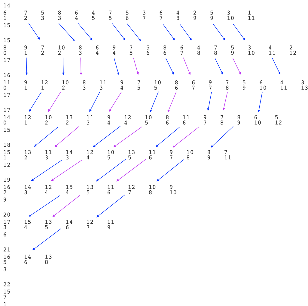
Fig. 3. Thresholds for intertwiners (9, 5) \otimes (6, 2) \rightarrow (v_1, v_2) . Each line (levels k^{min} = 14 to k^{max} = 22 ) lists those irreps v (components given vertically) for which the multiplicity increases at the chosen level, i.e., for which a new coupling appears. The total number of new couplings at a given level is also given on the left. Same irreps for which there is a multiplicity increase are connected by arrows. The number of arrows with the same color gives the u_{pj} of sect. 5.2.3: at level k = 18 , i.e., p = k - k^{min} + 1 = 5 there are 5 irreps that are not hit by any arrowhead ( u_{50} = 5 ), 4 hit by a blue arrow ( u_{51} = 4 ), and ( u_{52} = 3 ) hit by a red arrow, the total multiplicity increasing of 5 + 4 + 3 = 12 . (For interpretation of the references to color in this figure, the reader is referred to the web version of this article.)
