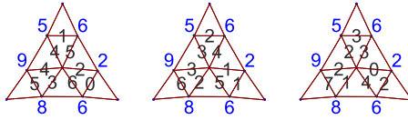
Fig. 1. The three couplings of (9, 5) \otimes (6, 2) \rightarrow (8, 6) using the O-blade model.
