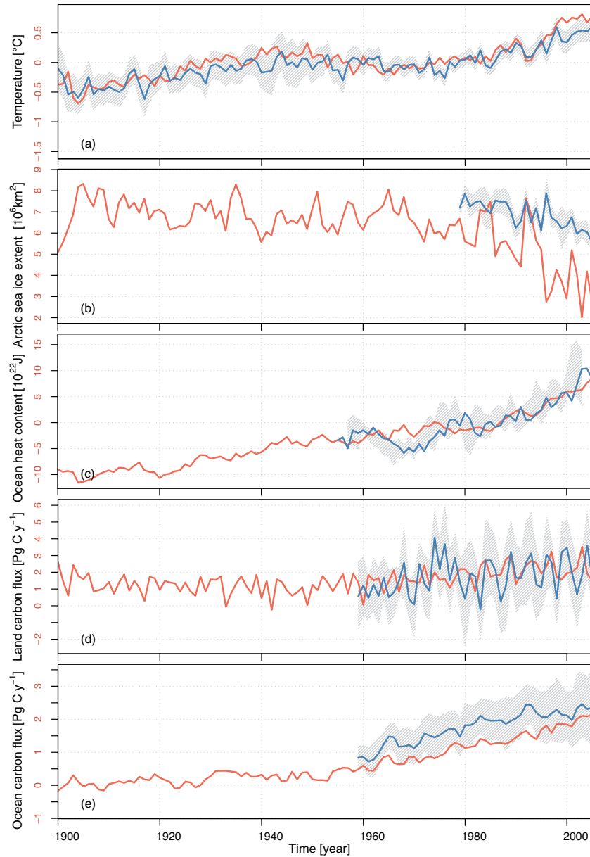
Figure 19. Time series of various climate indices as monitored from available observations (blue solid line) and as simulated by CNRM-ESM1 (red solid line) since 1901 with global near-surface temperature (a), September Arctic sea-ice extent (b), 0–2000 m ocean heat content (c), land carbon flux (d) and ocean carbon flux (e). Hatching represents the \pm 2\sigma estimated from the ensemble deviation between the 100 members of the HadCRUT4 database (Morice et al., 2012) for near-surface temperature, the standard deviation between two National Snow and Ice Data Center estimates (Fetterer et al., 2002; Comiso, 1999) and Hadisst (Rayner et al., 2003) databases, the pentadal variability of the observed ocean heat content (Levitus et al., 2012) and spread between Global Carbon Project reconstructions for both land and ocean (Le Qu  r   et al., 2014). For both OCS and LCS, positive (negative) fluxes indicate an uptake (outgassing) of \text{CO}_2 .
