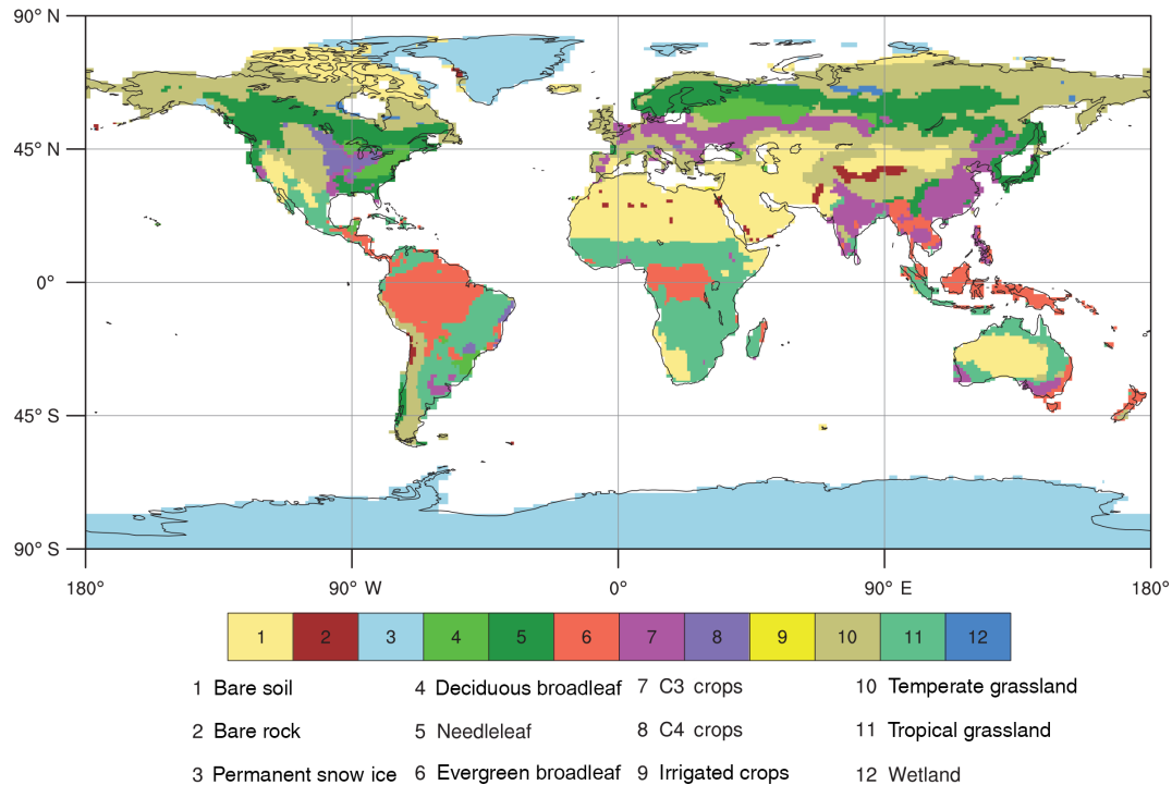
Figure 1. Fraction of dominant vegetation type as prescribed in SURFEX. This fraction results from aggregation of the various ECO-CLIMAP’s vegetation types at 1 km resolution over the T127 CNRM-ESM1 horizontal grid ( \sim 1.4^\circ nominal horizontal resolution).
