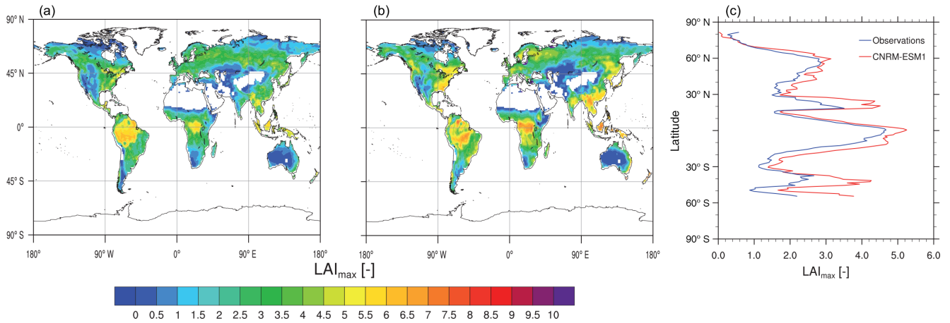
Figure 17. Composite of yearly maximum of leaf area index (LAI max ) as estimated from AVHRR satellite observations of Zhu et al. (2013) (a) and as simulated by CNRM-ESM1 (b) over 1986–2005. Panel (c) represents the zonal-average LAI max in function of latitude for both observation-based estimates (in blue) and CNRM-ESM1 (in red).
