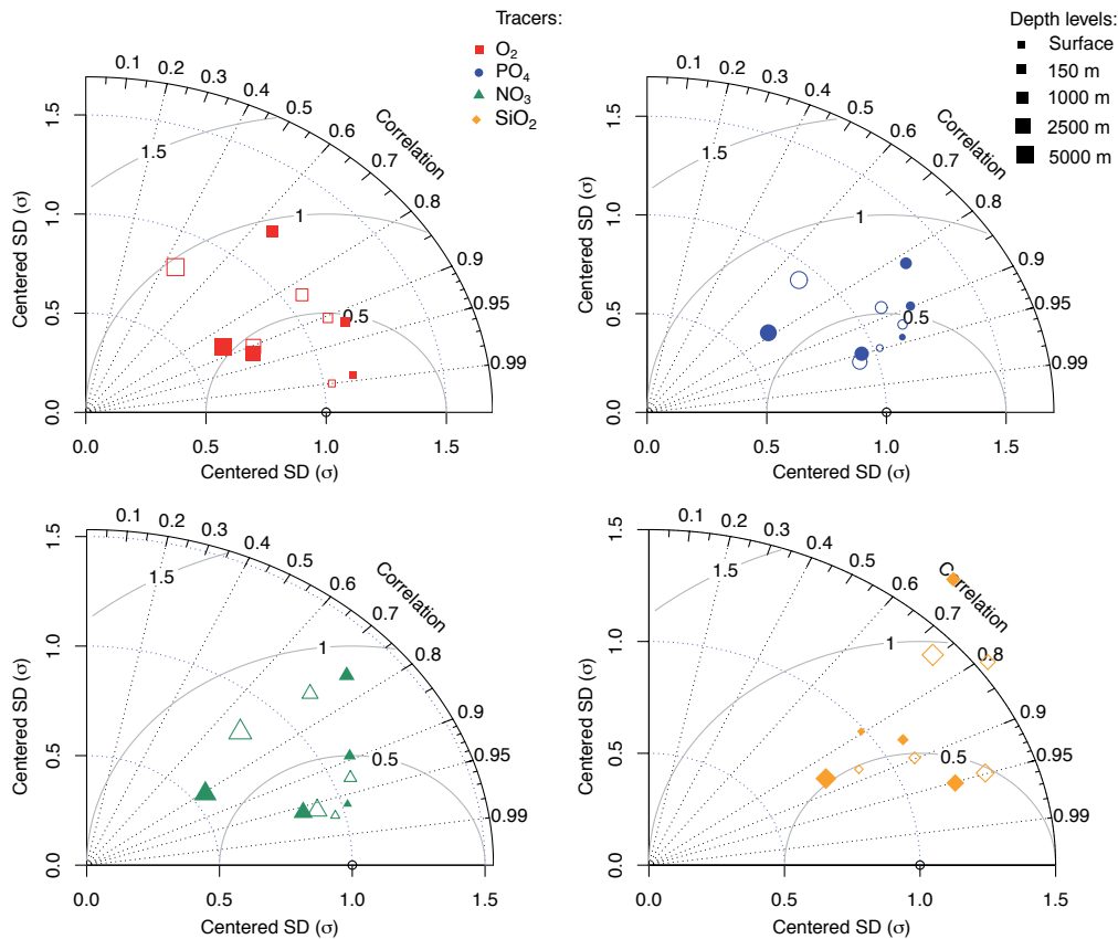
Figure 14. Taylor diagrams showing the correspondence between model results and observations for CNRM-ESM1 and CNRM-CM5.2 (S  ferian et al., 2013). Climatological distribution over 1986–2005 of simulated oxygen ( O_2 ), phosphate ( PO_4 ), nitrate ( NO_3 ) and silicate ( SiO_2 ) concentrations are assessed against WOA2013 data product. Filled and empty symbols indicate skills for CNRM-ESM1 and CNRM-CM5, respectively. The size of the symbols indicates the depth at which statistics have been computed.
