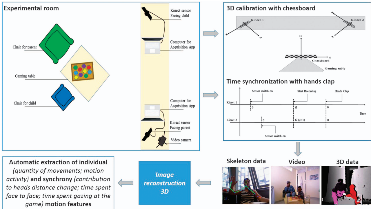
Figure 1. Experimental setup for capture and extraction of two-dimensional plus three-dimensional (2D+3D) motion feature during mother-infant early interaction. Two Kinect cameras (one for the mother and one for the infant) record the interaction. To permit 3D reconstruction, the video data are synchronized for time through hand clapping and spatial 3D calibration is possible through a chessboard used at the beginning of the recording. The 2D images, 3D images and skeleton are recorded during infant-mother interaction. After the 3D reconstruction, several 2D+3D motion features are extracted at both individual (quantity of movements, motion activity) and synchrony levels (contribution to heads distance change; time spent face to face; time spent gazing at the game; overlap ratio; pause ratio; synchrony ratios).
