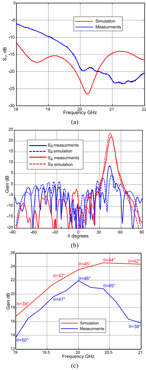
Fig. 10. (a) Measured and simulated reflection coefficients. (b) Measured and simulated copolarization ( E_\theta ) and cross polarization ( E_\phi ) components. (c) Measured and simulated gains in the frequency range spanning between 19 and 21 GHz. The main beam direction is also indicated.
