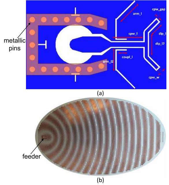
Fig. 11. (a) Directional feeder geometry: cpw_l = 2.25 mm, cpw_w = 0.3 mm, arm_l = 1.9 mm, arm_{l2} = 1.5 mm, bend = 45^\circ , dip_l = 1.1 mm, dip_{l2} = 0.87 mm, and coupl_l = 0.8 mm, via hole diameter = 0.4 mm, pitch = 0.6 mm. (b) Alternative LP antenna final design with nonuniform modulation index.
