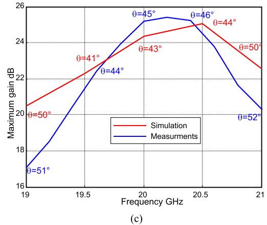
Fig. 9. (a) Measured and simulated reflection coefficients. (b) Measured and simulated copolarization Right-hand Circular Polarization and cross polarization Left-hand Circular Polarization components. (c) Measured and simulated gains in the frequency range spanning between 19 and 21 GHz. The main beam direction is also indicated.
