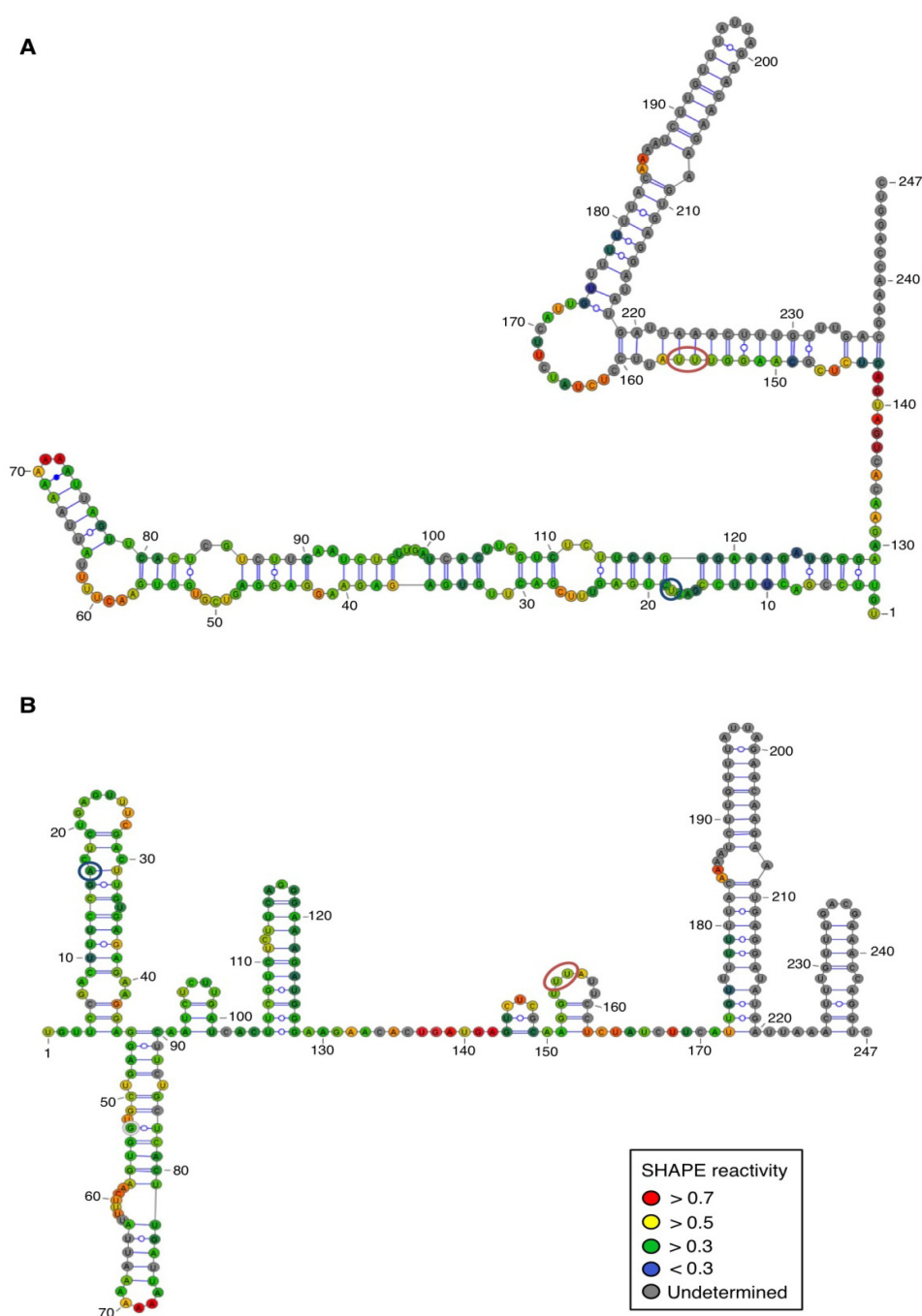
Figure 4. Secondary structure models of ASBVd (+) based on the SHAPE analysis. (A) and (B) are the two secondary structure models proposed for ASBVd (+). The color of the circle surrounding each nucleotide reveals their relative reactivity to 1M7 in the presence of 10 mM Mg^{2+} , as mentioned in the box. High reactivity reflects single-stranded region, while paired nucleotides are not reactive. Nucleotides for which the reactivity could not be determined are shown in grey and correspond to the primer binding site, or to nucleotide right 3' to the primer for which the electrophoresis resolution is not good enough, or to RT stops. The same experiments were carried out without Mg^{2+} and differences in reactivity are represented on the scheme: nucleotides circled in red show enhanced reactivity in the presence of Mg^{2+} , and those in blue are less reactive. The models were designed using VaRNA [31].
