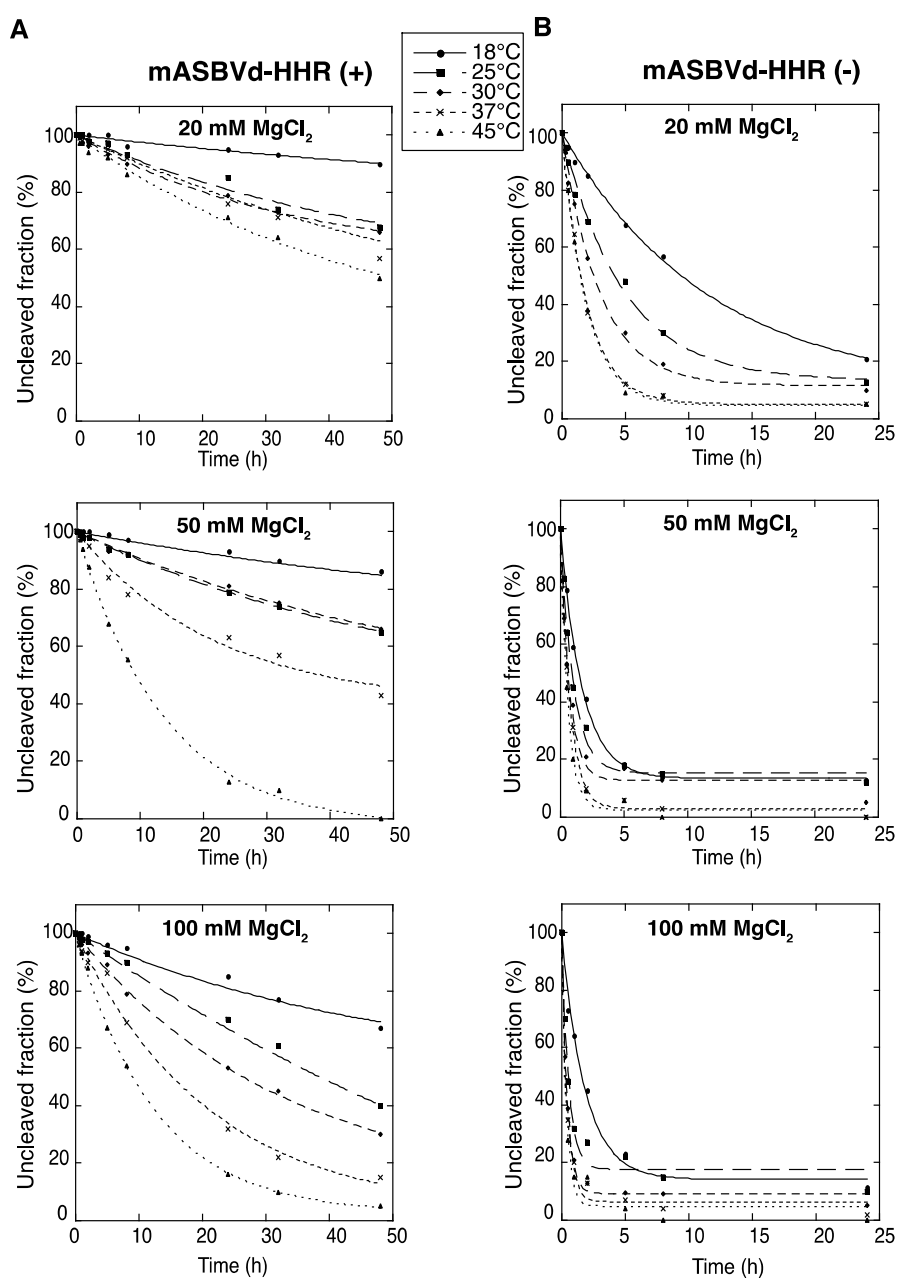
Figure 1. Self-cleavage kinetics of purified monomeric ASBVd-HHR (+) (A) and ASBVd-HHR (−) (B) transcripts. Self-cleavage reactions were carried out at 18 °C, 25 °C, 30 °C, 37 °C and 45 °C in buffers containing either 20 mM, 50 mM or 100 mM MgCl 2 . Aliquots were removed at different time up to 48 h for ASBVd (+) (panels A) and 24 h for ASBVd (−) (panels B), quenched with an excess of stop solution and separated on 10% polyacrylamide gels. After ethidium bromide staining, the percentage of uncleaved molecules was quantified using the ImageJ Software [25]. Quantitative data were fitted to multiexponential curves with the KaleidaGraph program (Synergy Software, Reading, PA, USA).
