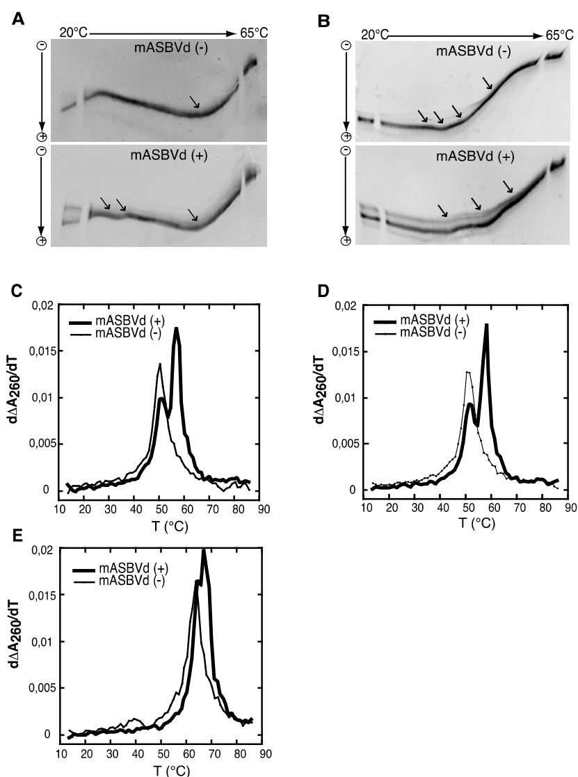
Figure 2. Temperature gradient gel electrophoresis (TGGE) and melting curves of mASBVd (+) and mASBVd (−) transcripts. (A) TGGE analysis performed by native 8% PAGE in 0.2× TBE buffer. (B) TGGE analysis performed by native 8% PAGE in 0.2× TB buffer containing 20 \mu\text{M} magnesium acetate. Migration was monitored between 20 °C and 65 °C. The arrows denote the transition temperatures. Derivative absorbance melting profiles were determined either in 150 mM KCl and 10 mM sodium cacodylate (pH 7.2) (C) or with, in addition, 100 \mu\text{M} \text{MgCl}_2 (D) or 1 M NaCl (E). The first derivative profiles ( d\Delta A_{260}/dT ) are shown with a thick curve for mASBVd (+) and a thin curve for mASBVd (−).
