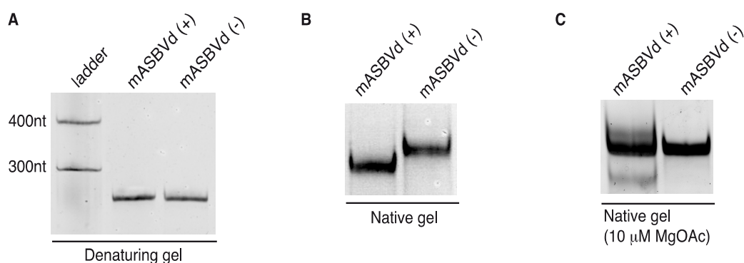
Figure 3. Electrophoretic mobility of mASBVd RNAs. The mASBVd (+) and mASBVd (−) transcripts were separated on 8% PAGE gels in 1× TBE buffer under denaturing (A) and native (B) conditions. The RiboRuler™ low range RNA ladder (Fermentas, Thermo Fisher Scientific Inc., Waltham, MA, USA) was loaded in parallel with mASBVd (+) and (−) into the denaturing gel (A). (C) RNA transcripts were analyzed on 8% PAGE native gel in 1× TB buffer containing 10 μM magnesium acetate.
