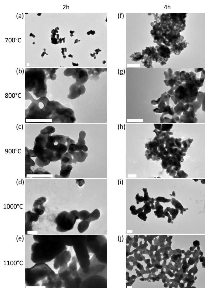
Fig. 3 TEM images of \text{Eu}^{3+} , \text{Ti}^{4+} , \text{Mg}^{2+} doped \text{Gd}_2\text{O}_2\text{S} nanoparticles depending on annealing treatment under argon: (a) 700°C-2h; (b) 800°C-2h; (c) 900°C-2h; (d) 1000°C-2h; (e) 1100°C-2h; (f) 700°C-4h; (g) 800°C-4h; (h) 900°C-4h; (i) 1000°C-4h; (j) 1100°C-4h. All scale bars are 100 nm.
