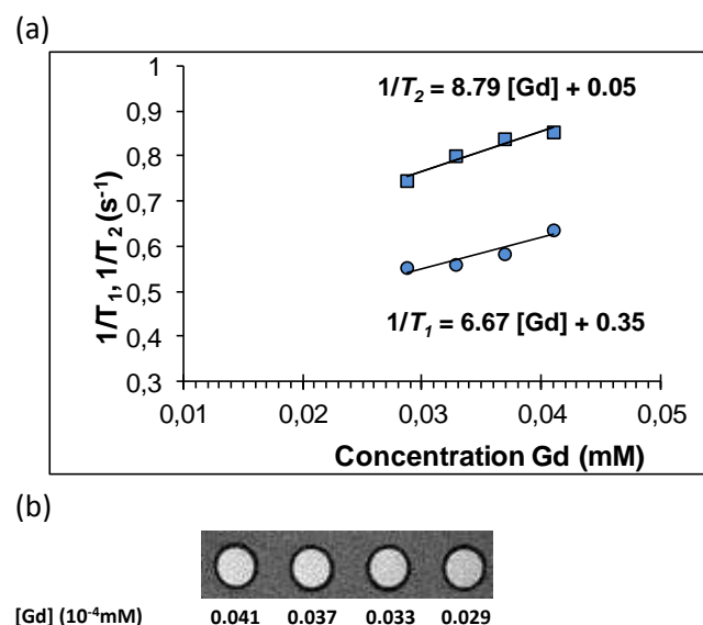
Fig. 7 (a) ^1H relaxation rates measured with Gd_2O_2S: Eu5\%, Ti1\%, Mg8\% aqueous suspensions. (b) Resulting MR-images (1.5 T, 21^\circ C ; T_2 -weighted fast spin-echo; TR, 400 ms; TE, 10.8 ms).
