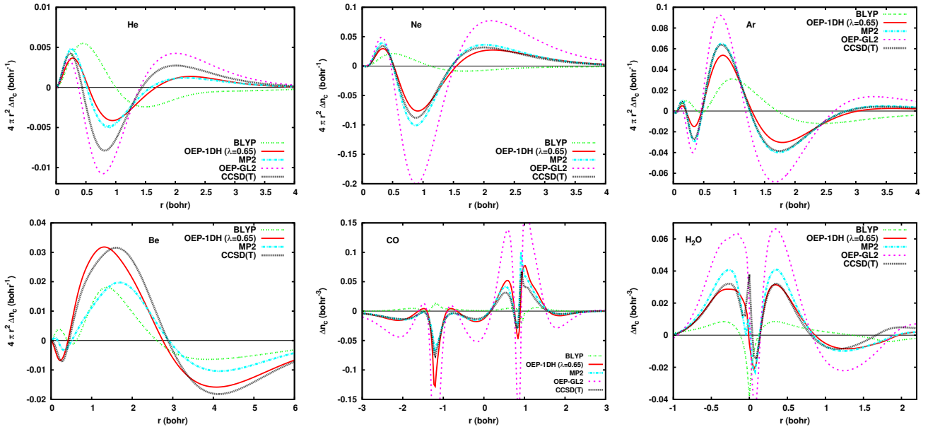
FIG. 6. Correlated density calculated with the OEP-1DH approximation using the BLYP functional at the recommended value \lambda = 0.65 , and at the extreme values \lambda = 0 (standard BLYP) and \lambda = 1 (OEP-GL2). The reference correlated densities are calculated with CCSD(T). For comparison, correlated densities calculated with standard MP2 are also shown. For Be, the OEP-GL2 calculation is unstable. For CO, the potential is plotted along the direction of the bond with the C nucleus at -1.21790 bohr and the O nucleus at 0.91371 bohr. For H 2 O, the potential is plotted along the direction of a OH bond with the O nucleus at 0.0 and the H nucleus at 1.81225 bohr.
