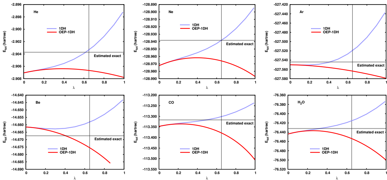
FIG. 1. Total energies calculated with the 1DH and OEP-1DH approximations with the BLYP functional as a function of \lambda . The estimated exact total energies are from Ref. 67 for He, Be, Ne, Ar, and from Ref. 68 for CO and H 2 O. The vertical lines correspond to \lambda = 0.65 , i.e. the value recommended for 1DH with the BLYP functional in Ref. 21. For Be, the OEP-1DH calculations are unstable for \lambda > 0.86 .
