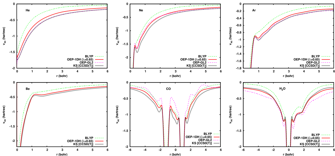
FIG. 4. Exchange-correlation potentials calculated with the OEP-1DH approximation [Eq. (9)] using the BLYP functional at the recommended value \lambda = 0.65 , and at the extreme values \lambda = 0 (standard BLYP) and \lambda = 1 (OEP-GL2). The reference potentials were calculated by KS inversion of the CCSD(T) densities. For Be, the OEP-GL2 calculations are unstable. For CO, the potential is plotted along the direction of the bond with the C nucleus at -1.21790 bohr and the O nucleus at 0.91371 bohr. For \text{H}_2\text{O} , the potential is plotted along the direction of a OH bond with the O nucleus at 0.0 and the H nucleus at 1.81225 bohr.
