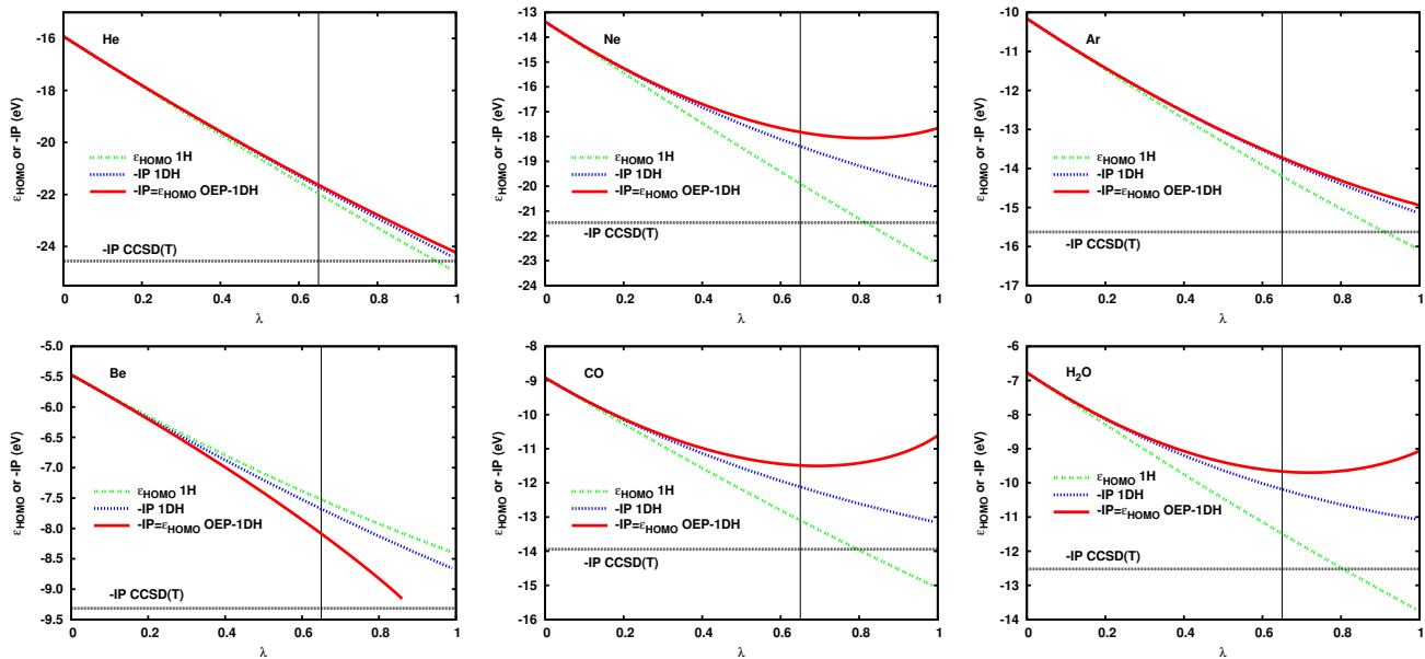
FIG. 2. HOMO orbital energies in the 1H approximation [Eq. (6)] and minus IPs in the 1DH [Eq. (28)] and OEP-1DH [Eq. (23)] approximations using the BLYP functional as a function of \lambda . The reference values were calculated as CCSD(T) total energy differences with the same basis sets. The vertical lines correspond to \lambda = 0.65 , i.e. the value recommended for 1DH with the BLYP functional in Ref. 21. For Be, the OEP-1DH calculations are unstable for \lambda > 0.86 .
