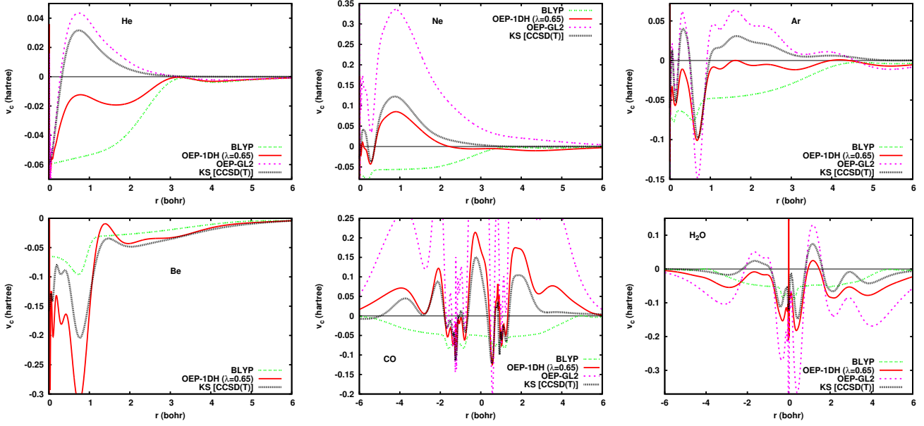
FIG. 5. Correlation potentials calculated with the OEP-1DH approximation [correlation terms in Eq. (9)] using the BLYP functional at the recommended value \lambda = 0.65 , and at the extreme values \lambda = 0 (standard BLYP) and \lambda = 1 (OEP-GL2). The reference potentials were calculated by KS inversion of the CCSD(T) densities. For Be, the OEP-GL2 calculation is unstable. For CO, the potential is plotted along the direction of the bond with the C nucleus at -1.21790 bohr and the O nucleus at 0.91371 bohr. For H 2 O, the potential is plotted along the direction of a OH bond with the O nucleus at 0.0 and the H nucleus at 1.81225 bohr.
