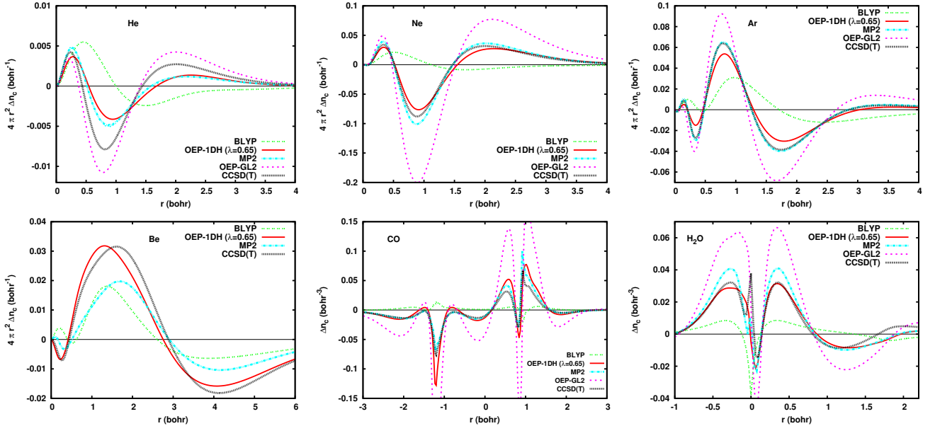
FIG. 7. Correlated density calculated with the OEP-1DH approximation using the BLYP functional at the recommended value \lambda = 0.65 , and at the extreme values \lambda = 0 (standard BLYP) and \lambda = 1 (OEP-GL2). The reference correlated densities are calculated with CCSD(T). For comparison, correlated densities calculated with standard MP2 are also shown. For Be, the OEP-GL2 calculation is unstable. For CO, the potential is plotted along the direction of the bond with the C nucleus at -1.21790 bohr and the O nucleus at 0.91371 bohr. For H 2 O, the potential is plotted along the direction of a OH bond with the O nucleus at 0.0 and the H nucleus at 1.81225 bohr.
