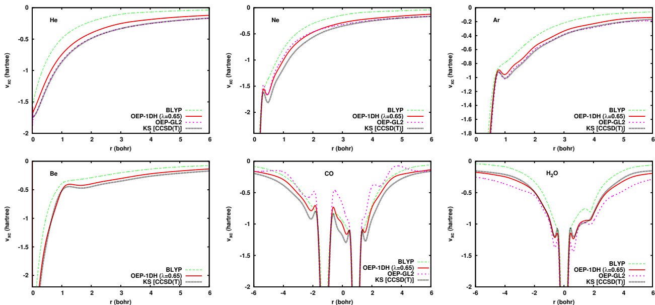
FIG. 5. Exchange-correlation potentials calculated with the OEP-1DH approximation [Eq. (9)] using the BLYP functional at the recommended value \lambda = 0.65 , and at the extreme values \lambda = 0 (standard BLYP) and \lambda = 1 (OEP-GL2). The reference potentials were calculated by KS inversion of the CCSD(T) densities. For Be, the OEP-GL2 calculations are unstable. For CO, the potential is plotted along the direction of the bond with the C nucleus at -1.21790 bohr and the O nucleus at 0.91371 bohr. For \text{H}_2\text{O} , the potential is plotted along the direction of a OH bond with the O nucleus at 0.0 and the H nucleus at 1.81225 bohr.
