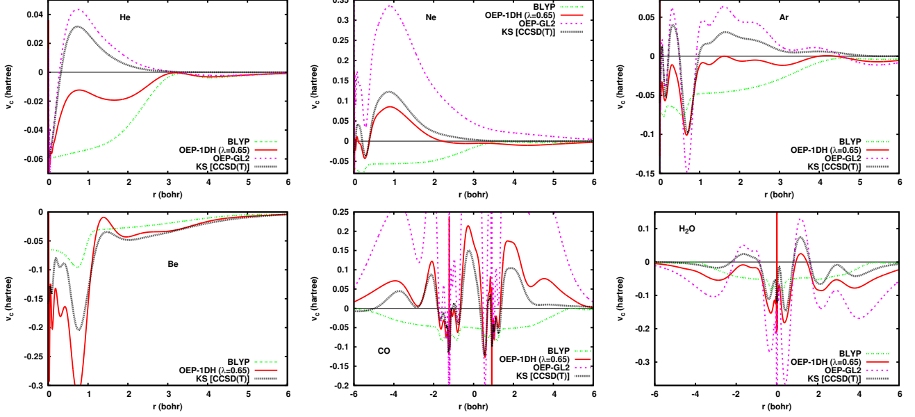
FIG. 6. Correlation potentials calculated with the OEP-1DH approximation [correlation terms in Eq. (9)] using the BLYP functional at the recommended value \lambda = 0.65 , and at the extreme values \lambda = 0 (standard BLYP) and \lambda = 1 (OEP-GL2). The reference potentials were calculated by KS inversion of the CCSD(T) densities. For Be, the OEP-GL2 calculation is unstable. For CO, the potential is plotted along the direction of the bond with the C nucleus at -1.21790 bohr and the O nucleus at 0.91371 bohr. For H 2 O, the potential is plotted along the direction of a OH bond with the O nucleus at 0.0 and the H nucleus at 1.81225 bohr.
