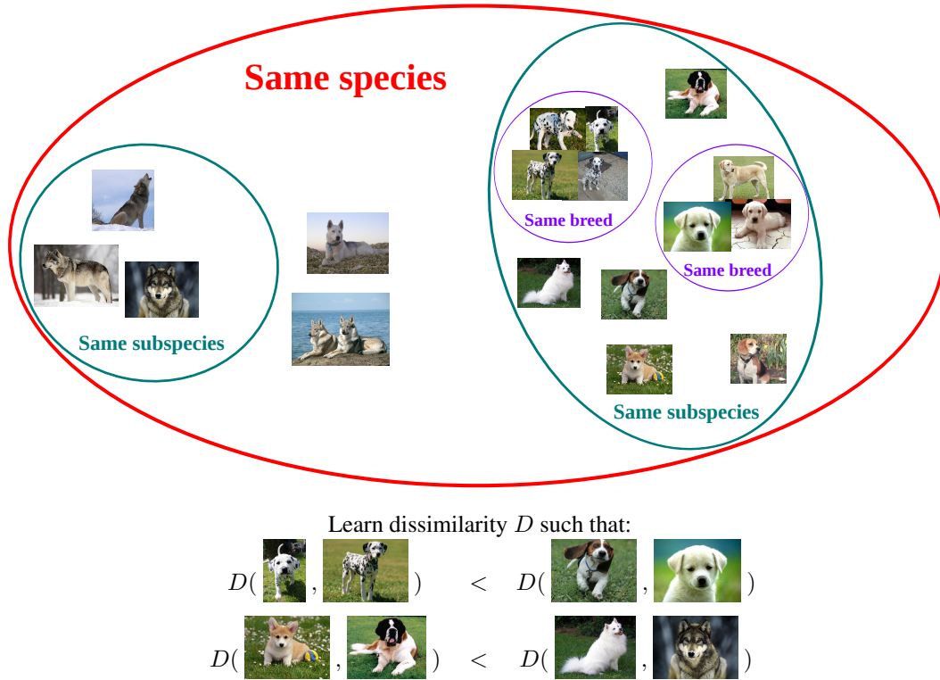
Fig. 2 Illustration of the quadruplet-wise (Qwise) strategy in a class taxonomy context. The goal is to learn a projection of animals of the same species such that members of the same breed are closer to each other than members from different breeds, and members from the same subspecies are closer to each other than member from different subspecies.
