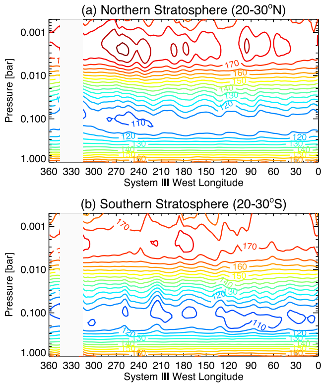
Fig. 17. Longitudinal cross-section of temperatures through stratospheric wave activity in Jupiter's northern and southern hemispheres observed by TEXES in December 2014. Contours are spaced every 5 K, and we see that northern and southern 2-mbar temperatures would be near-equal without the prominent northern wave.
