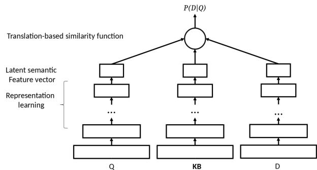
(b) The KB translation model
